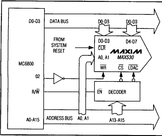
Figure 5. 4-Bit \mu P Interface
