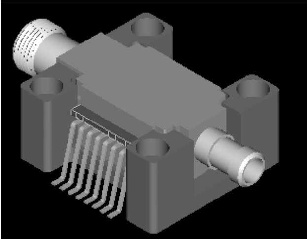
The R768 Receiver is manufactured in a 16-pin, pigtailed surface-mount metal package with a single-ended V-connector.
