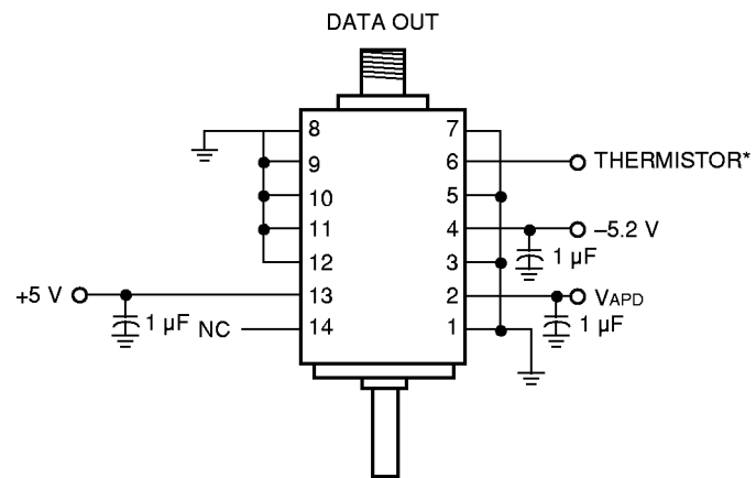
Figure 3. Circuit Diagram
