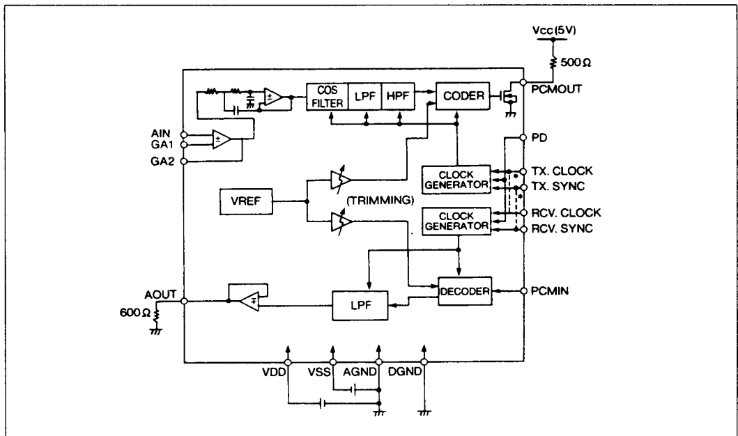
Figure 2 Block Diagram
