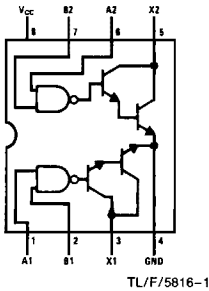
Top View Order Number DS1631J-8 or DS3631N
