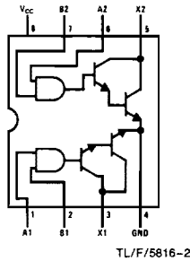
Top View Order Number DS1632J-8 or DS3632N See NS Package Number J08A or N08E
