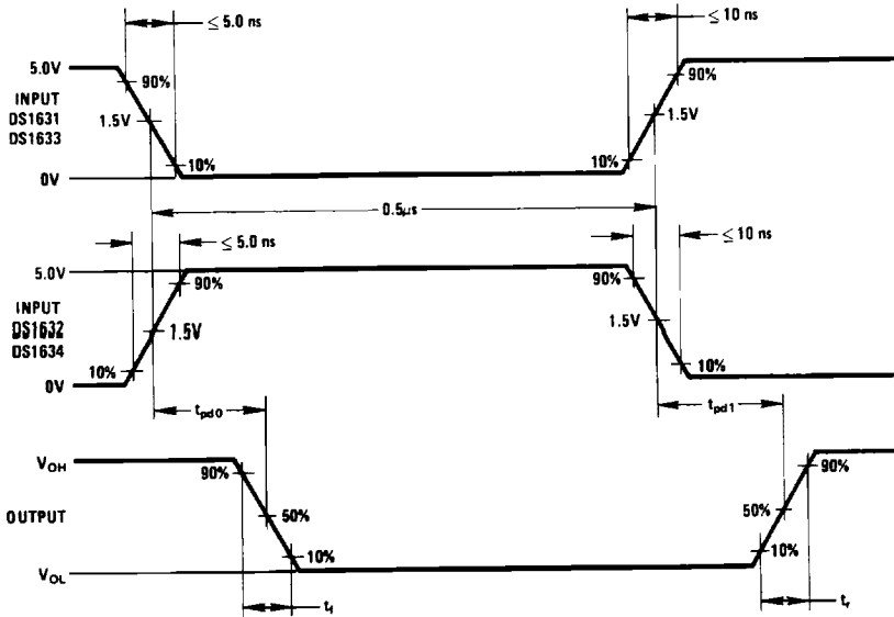
FIGURE 5. Switching Times
