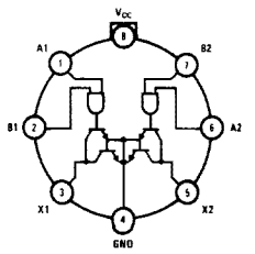
Top View (Pin 4 is electrically connected to the case.) Order Number DS1632H See NS Package Number H08C
