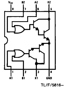
Top View Order Number DS1634J-8 or DS3634N
