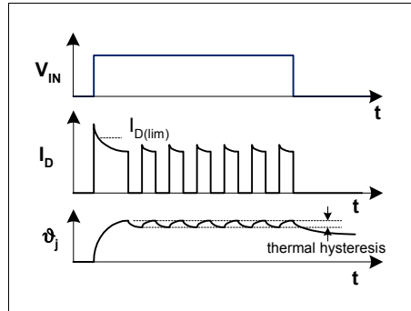
Figure 11 Short circuit
