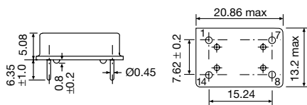
Figure 1) ECS-100 Series Side and Bottom views
