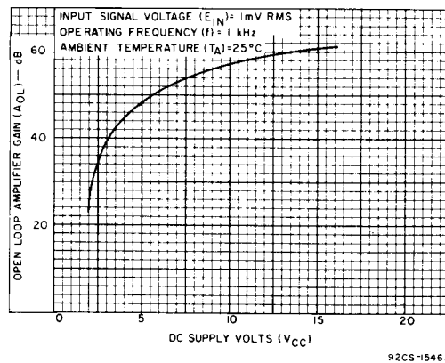
Fig. 7 - Typical amplifier gain vs DC supply voltage.
