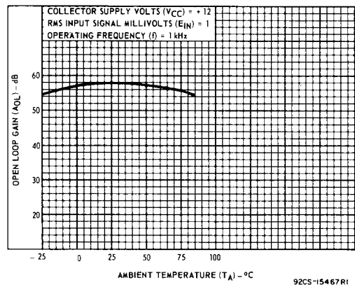
Fig. 8 - Typical open-loop gain vs ambient temperature.
