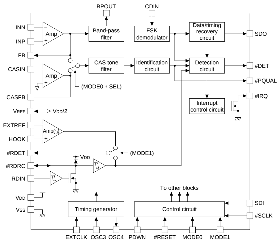
Figure 1.2.1 Block diagram
