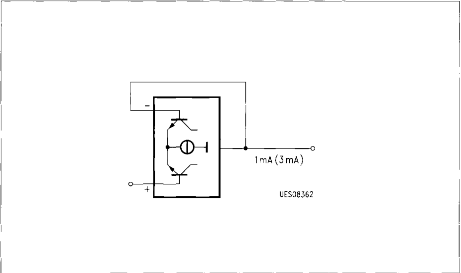
Figure 8 AF Outputs Pin 13/14/15/16
