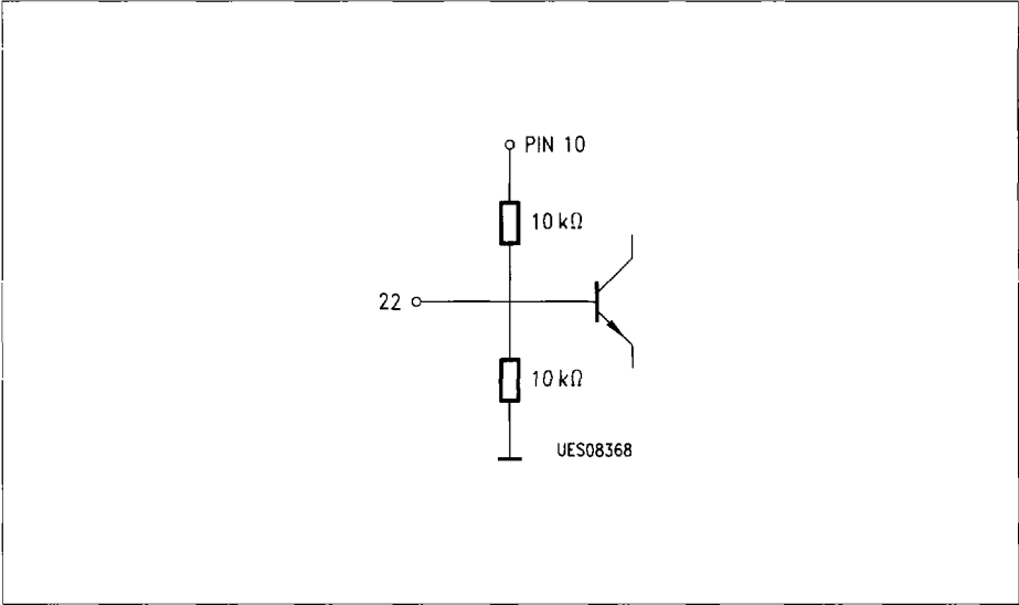
Figure 14 Bias for AF Operation Point Pin 22
