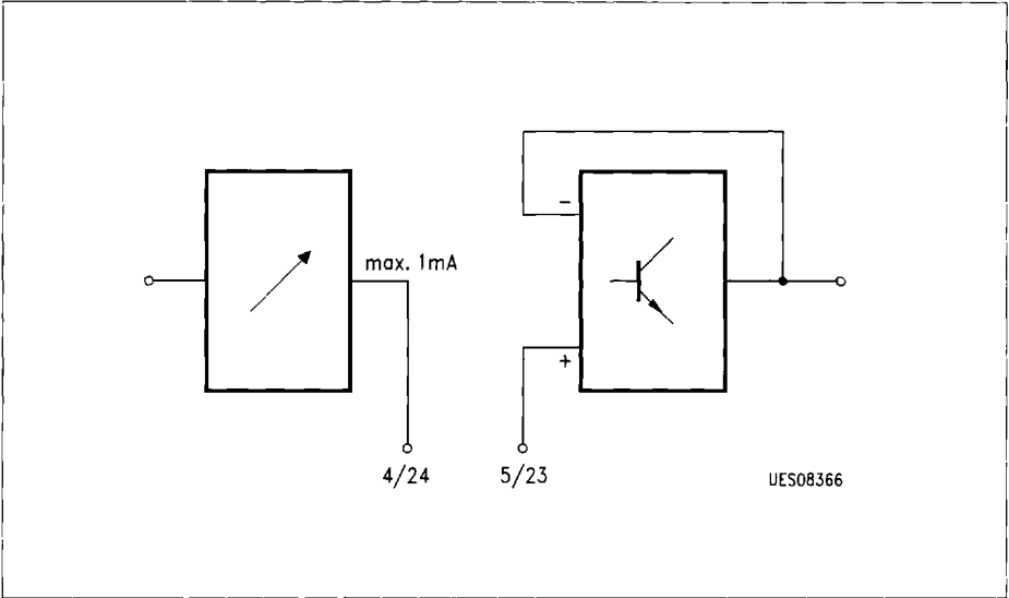
Figure 12 Loudness Pin 4/5/23/24
