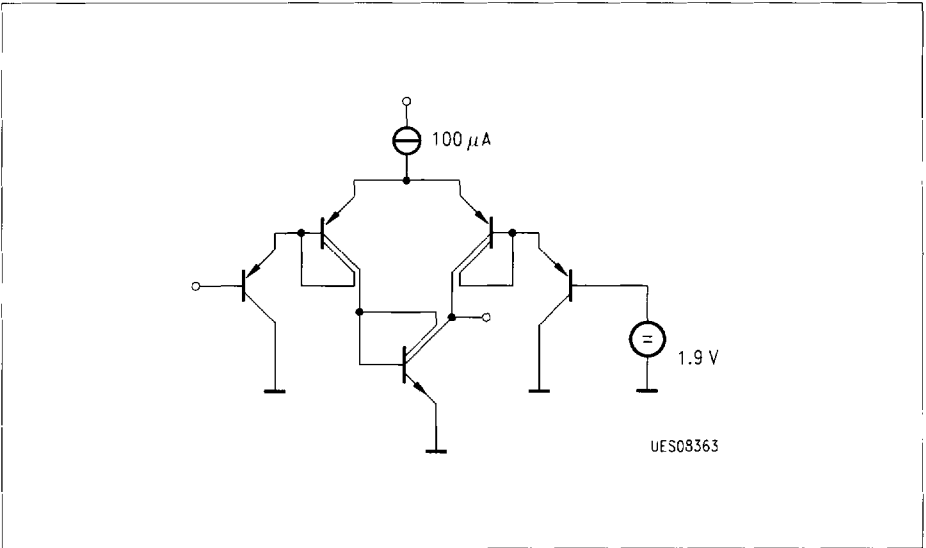
Figure 9 Mute Pin 7, I 2 C Bus SCL Pin 8
