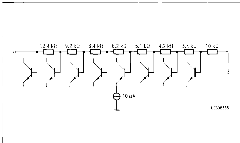
Figure 11 Corner Frequency Treble Pin 11/12
