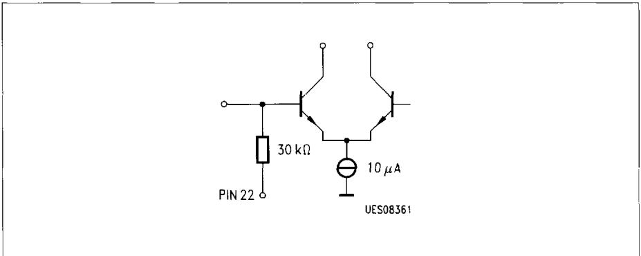
Figure 7 AF Inputs Pin 1/2/3/25/26/27/28
