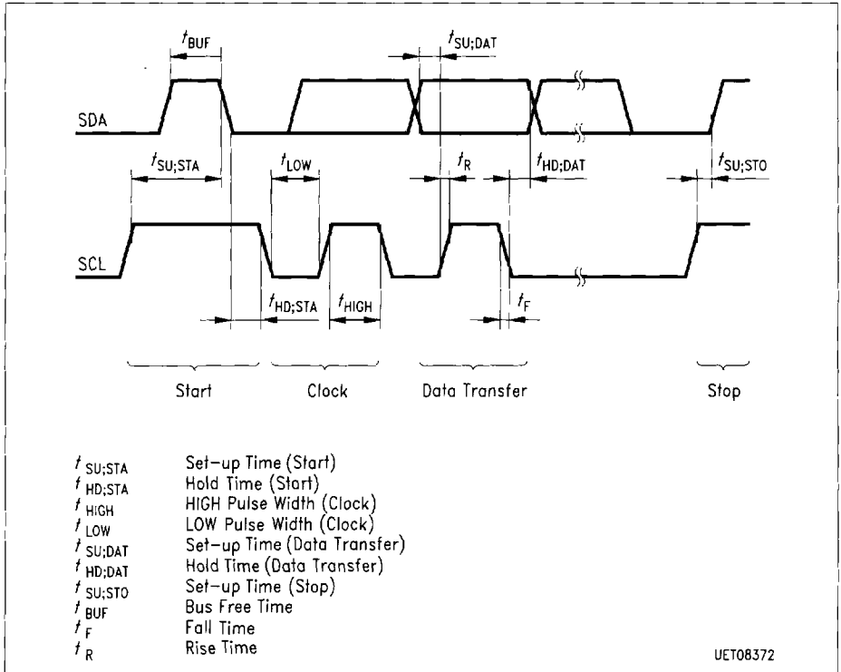
Figure 18 I 2 C Bus Timing
