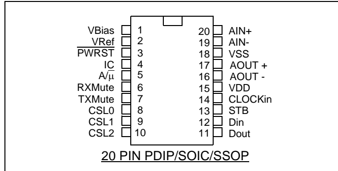
Figure 2 - Pin Connections
