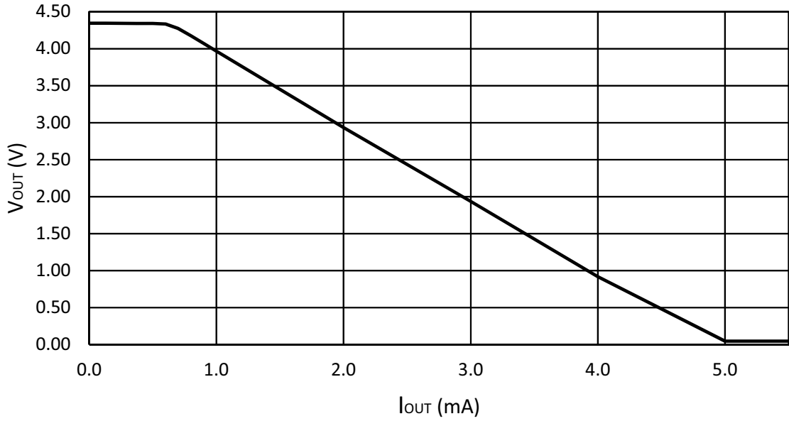
Figure 100. SLG46580 LDO Load Regulation, LOW POWER Mode, T = 25°C, V DD = 5V, V OUT = 4.35 V
