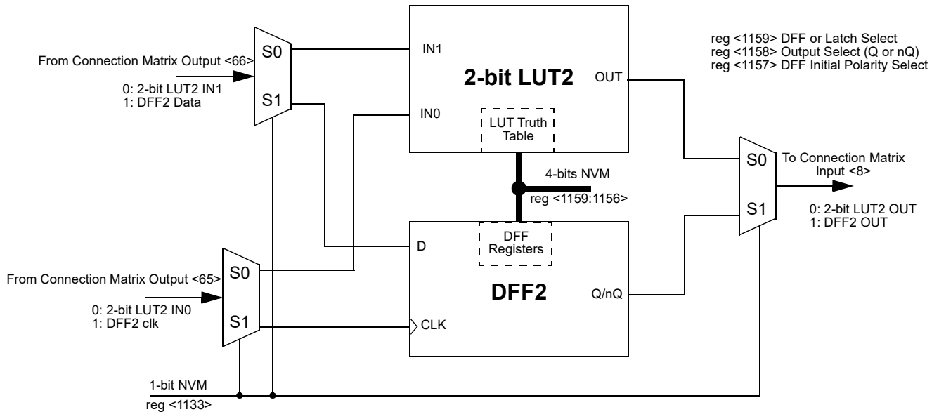
Figure 10. 2-bit LUT2 or DFF2
