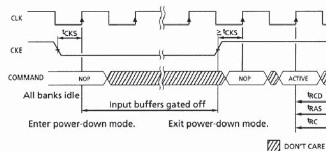
FIGURE 21: Power-Down
