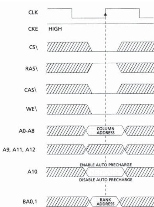
FIGURE 13: WRITE Command
