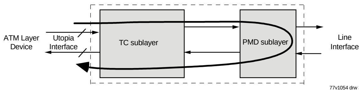
Figure 13 PHY Loopback
