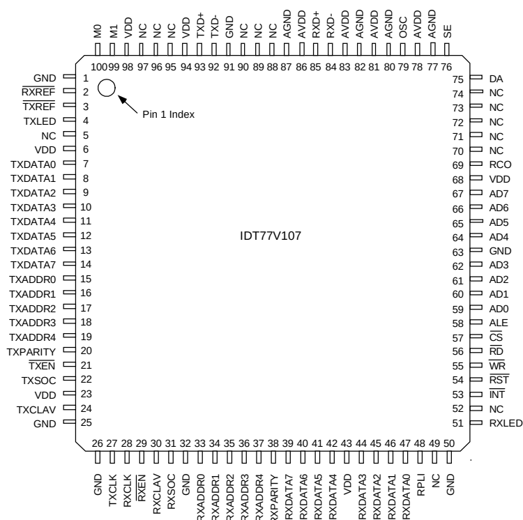
Figure 1 Pin Assignments
