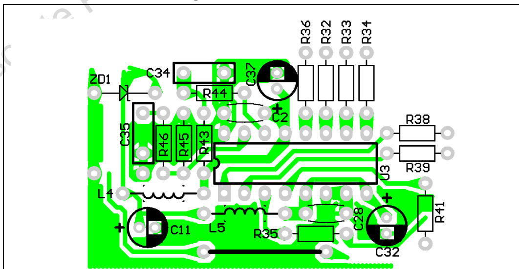
Figure 16: STV9936 - Zoom
