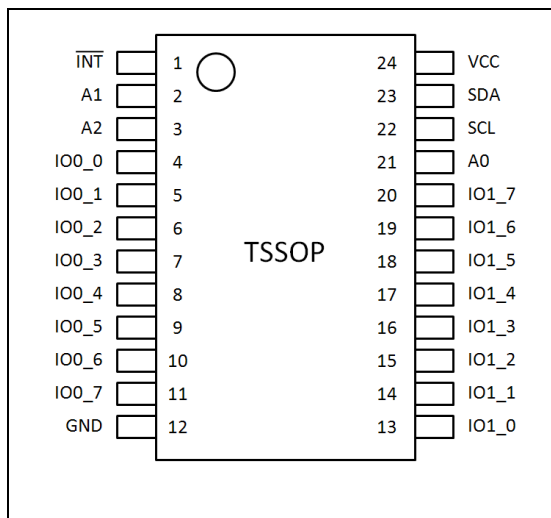
Figure 1:TSSOP24
