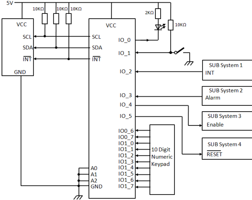
Figure 9: Typical application
