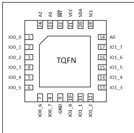
Figure 2:TQFN24
