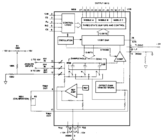
Figure 7. Unipolar Input Connections
