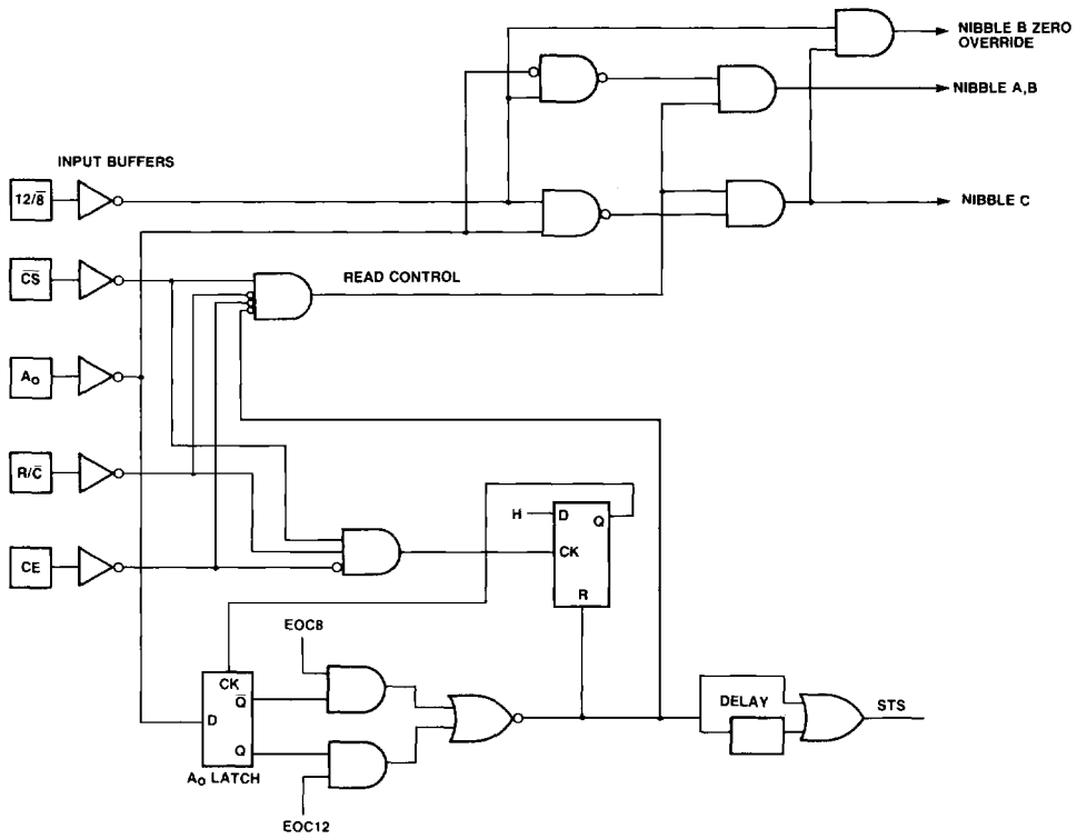
Figure 10. SP 674A Control Logic
