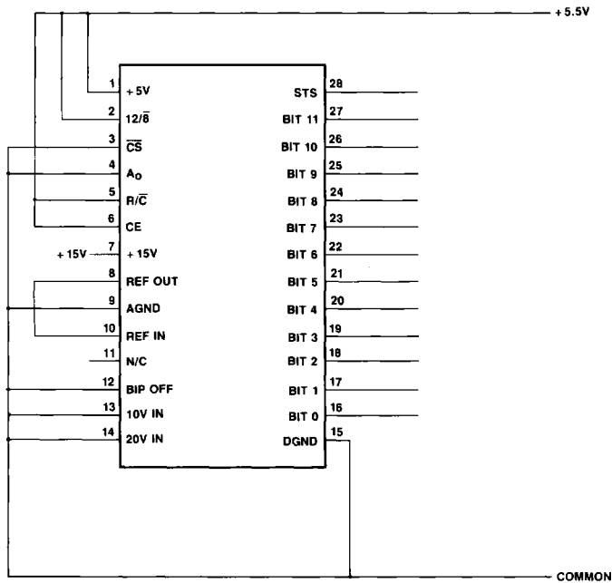
Figure 11. Burn-in Schematic
