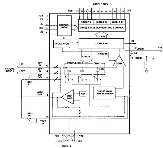
Figure 8. Bipolar Input Connections
