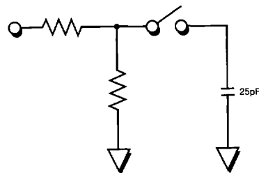
Figure 5. Sample and Hold Function
