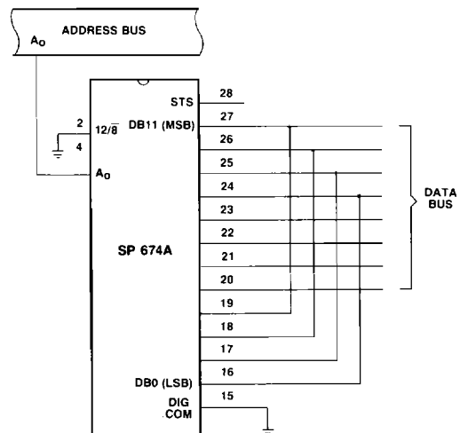
Figure 9. Interfacing the SP 674A to an 8-Bit Data Bus
