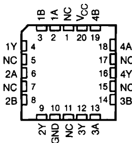
SN54ALS32, SN54AS32 ... FK PACKAGE (TOP VIEW)
