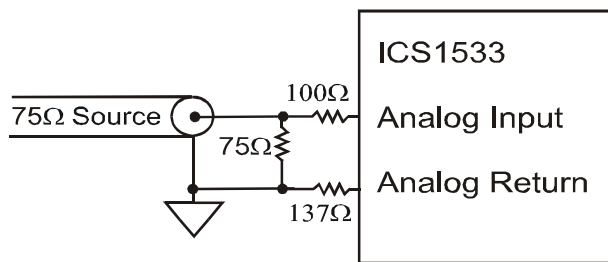
Figure 9-1. Recommended Termination
