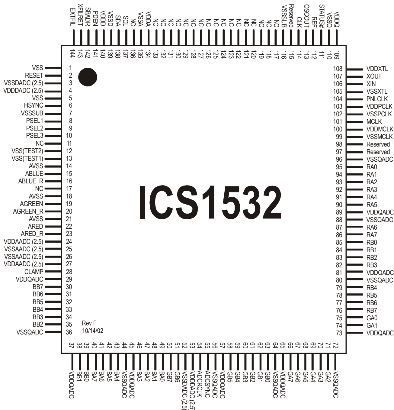
Figure 2-1. Pin Diagram
