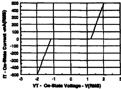
Figure 5. On-state terminal voltage vs. terminal current
