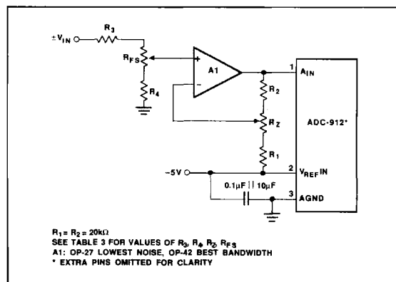
FIGURE 14: Noninverting Bipolar Analog Input Operation
