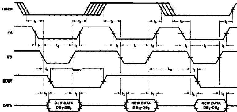
ROM MODE, TWO-BYTE READ DATA BUS STATUS
