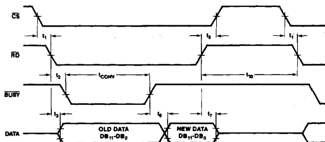
SLOW-MEMORY MODE, PARALLEL READ DATA BUS STATUS
