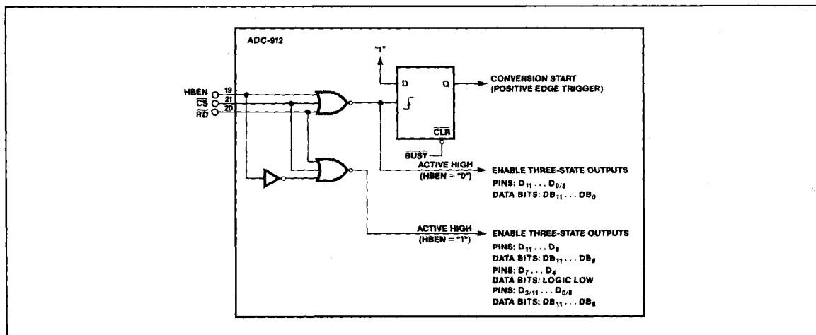
FIGURE 17: Internal Logic for Control Inputs \overline{CS} , \overline{RD} , and HBEN
