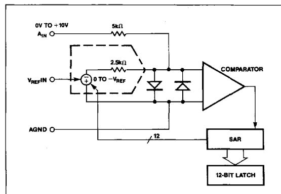
FIGURE 8: Simplified Analog Input Circuitry of ADC-912
