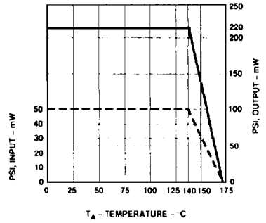
Figure 16. Dependence of Safety-Limiting Data on Ambient
