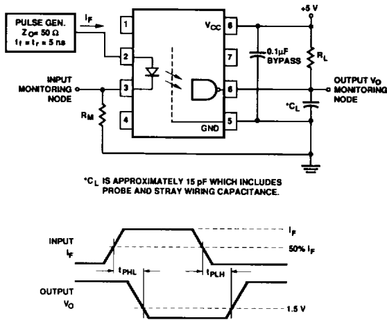
Figure 7. Test Circuit for t_{PHL} and t_{PLH} .
