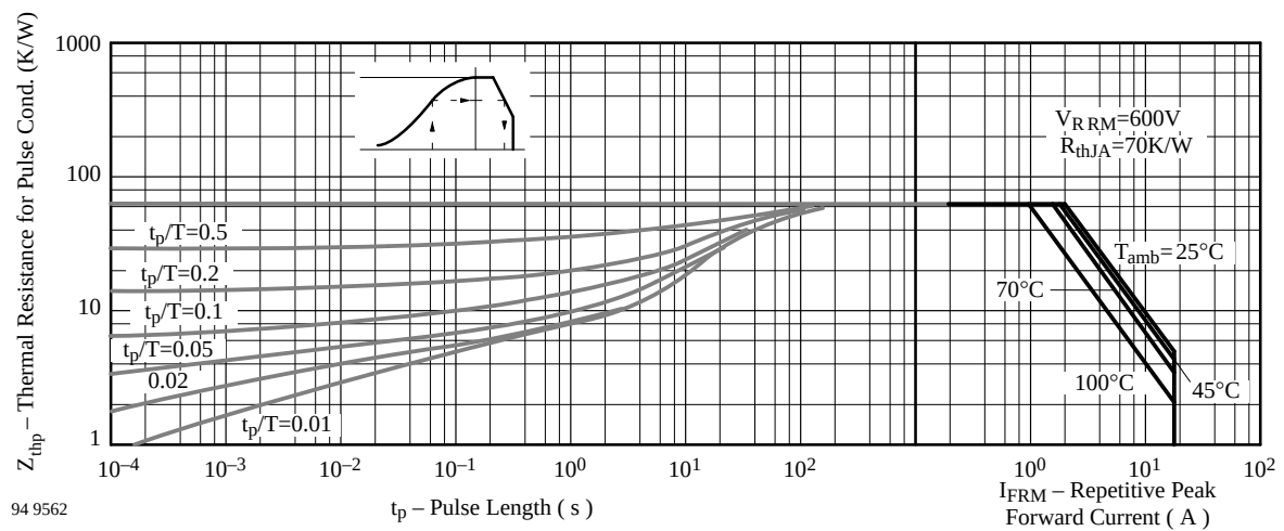
Figure 7. Thermal Response
