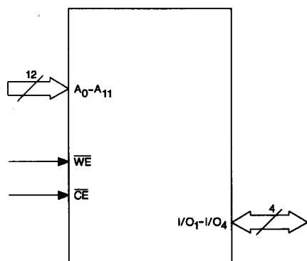
LOGIC SYMBOL
