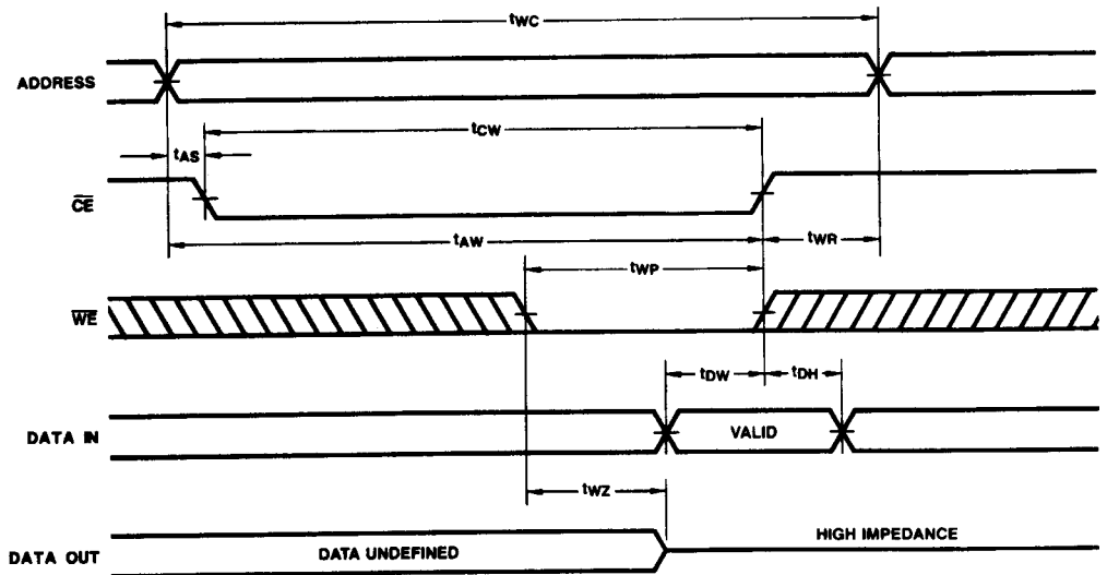
Write Cycle No. 2 — \overline{CE} Controlled
