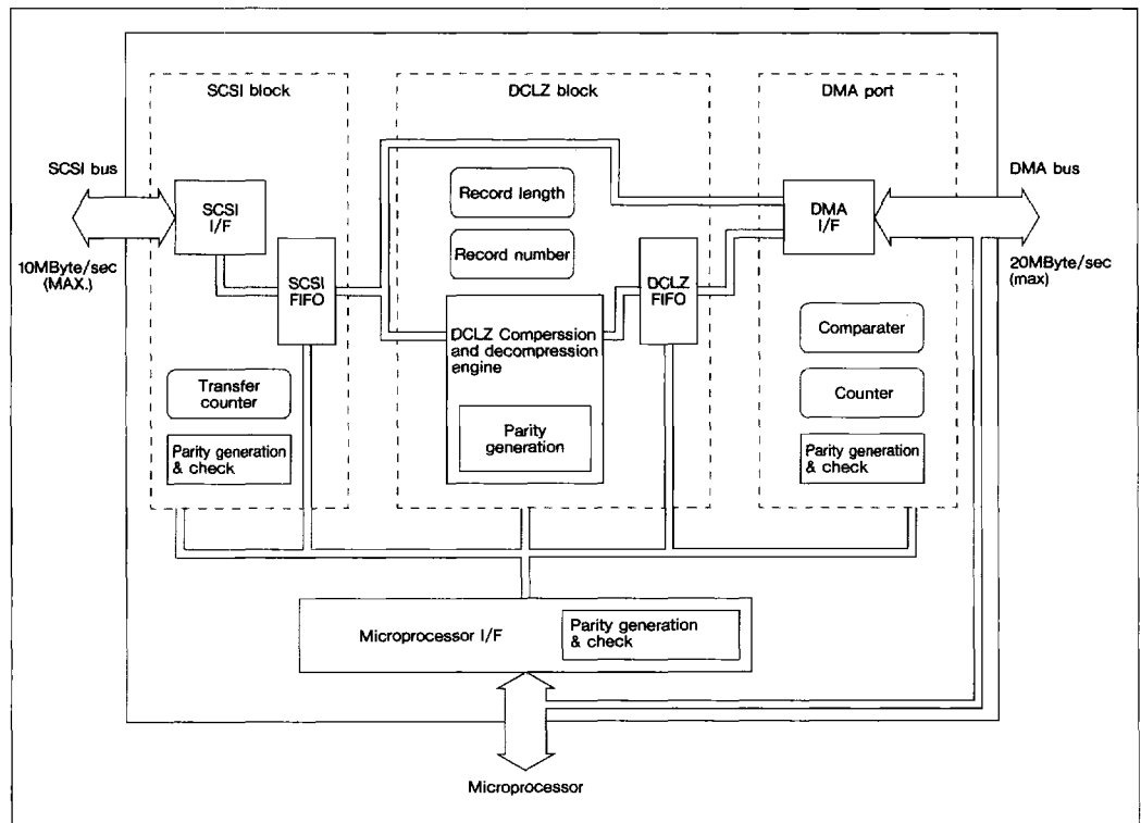
AK8311 BLOCK DIAGRAM
