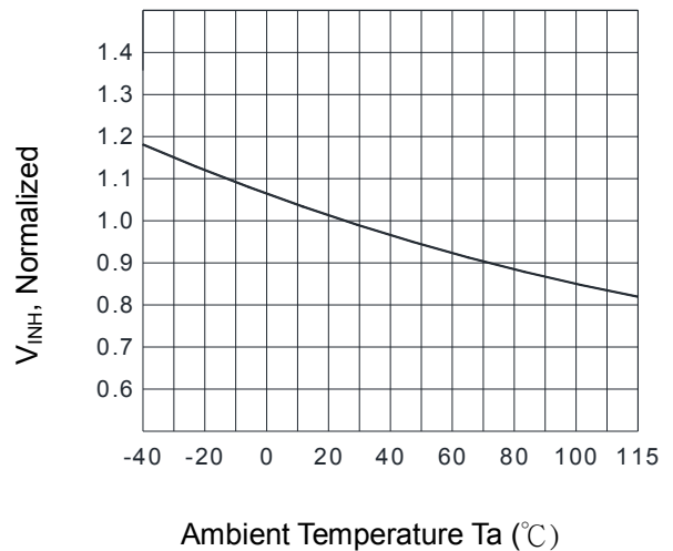
Fig.6 Inhibited Voltage vs. Ambient Temperature
