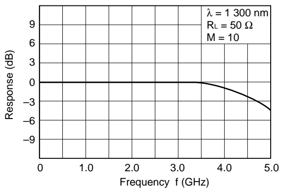
FREQUENCY RESPONSE
