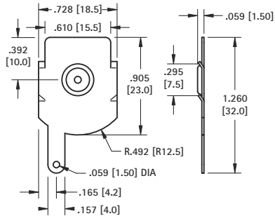
(+) POSITIVE BUTTON
