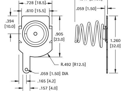
(-) NEGATIVE SPRING
