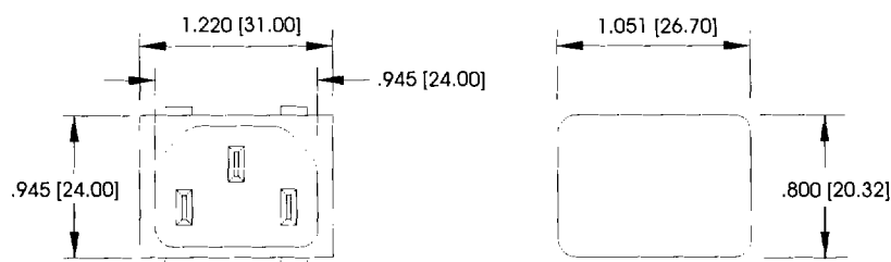
Panel Cut-Out
