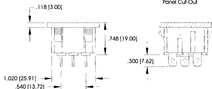
Panel Cut-Out
