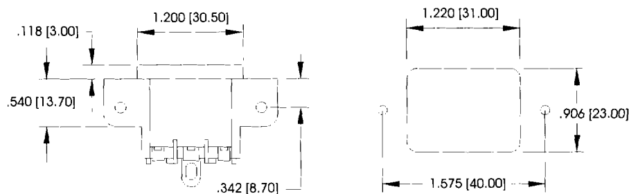
Panel Cut-Out
