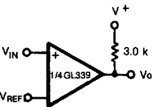
BASIC COMPARATOR
