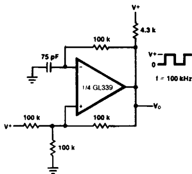
SQUAREWAVE-OSCILLATOR
