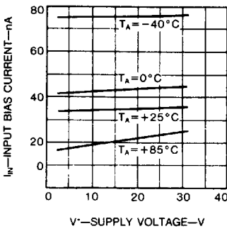
Figure 2—Input Current
