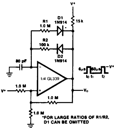
PULSE GENERATOR
