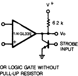
OUTPUT STROBING
