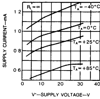
Figure 1—Supply Current
