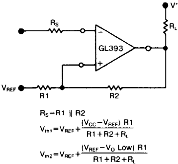
Figure 10-Comparator With Hysteresis
