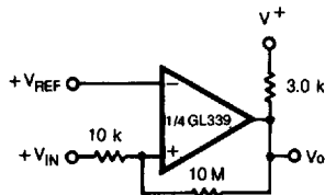
NON-INVERTING COMPARATOR WITH HYSTERESIS
