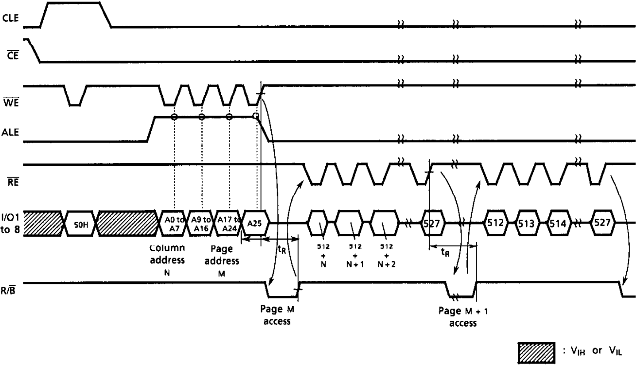
Sequential Read (3) Timing Diagram
