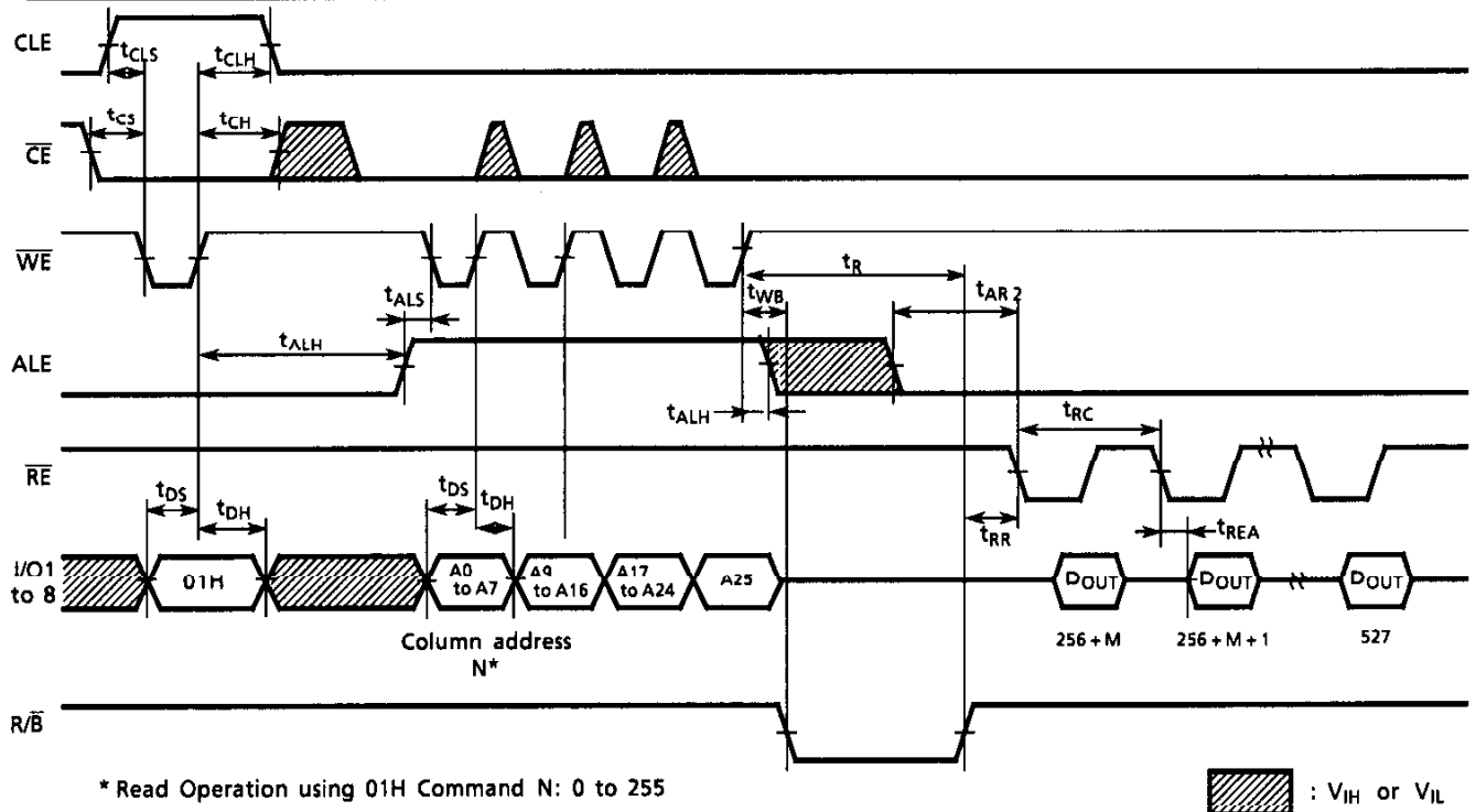
Read Cycle (2) Timing Diagram
