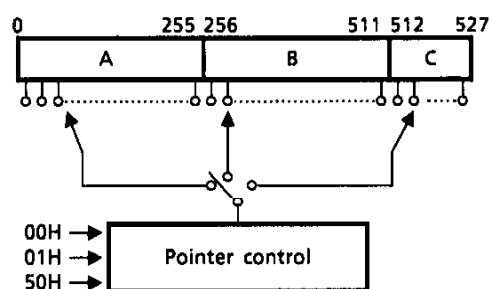
Figure 14. Pointer control
