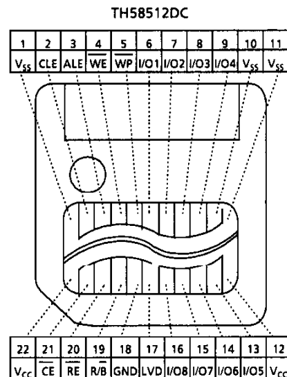
Figure 1. Pinout
