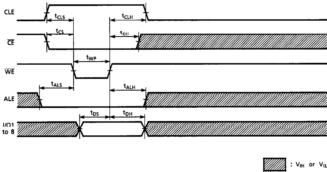
Command Input Cycle Timing Diagram
