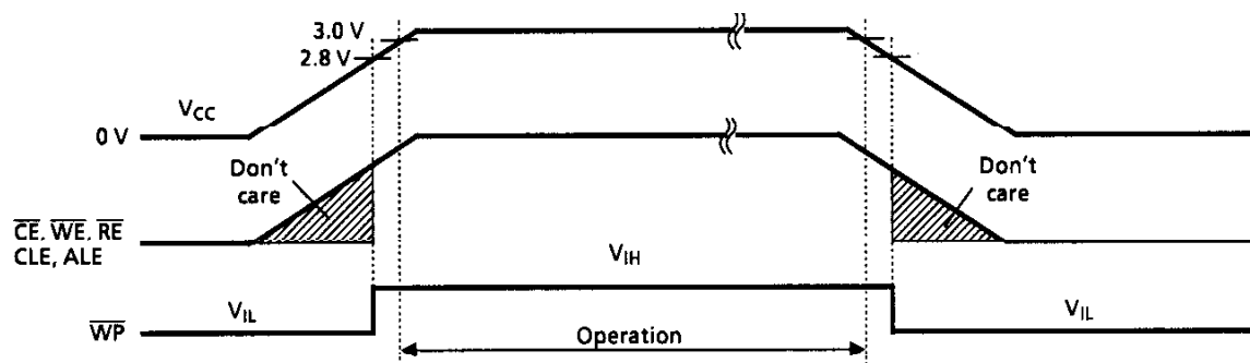
Figure 21. Power-on/off Sequence
