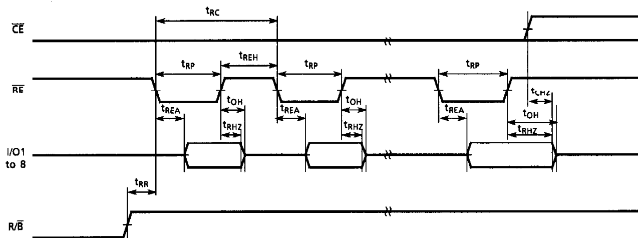
Serial Read Cycle Timing Diagram
