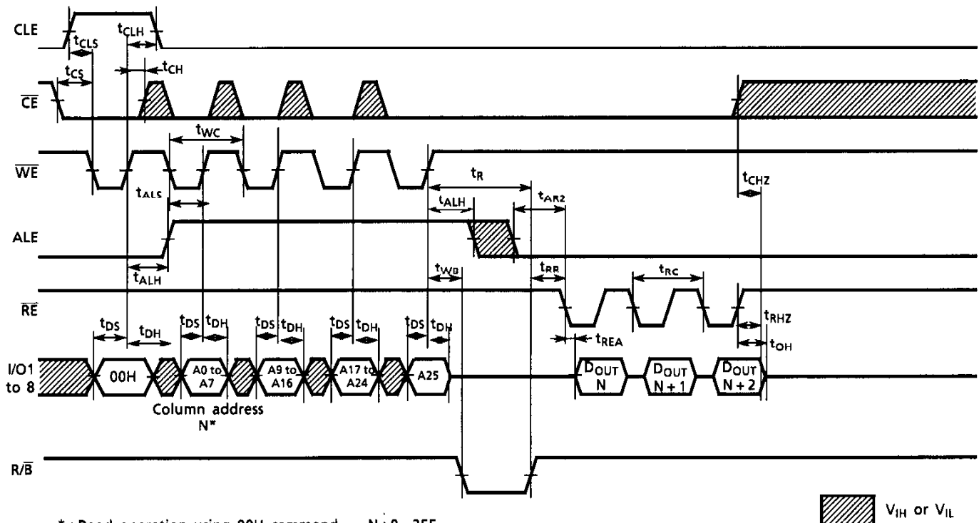
Read Cycle (1) Timing Diagram: When Interrupted by \overline{CE}
