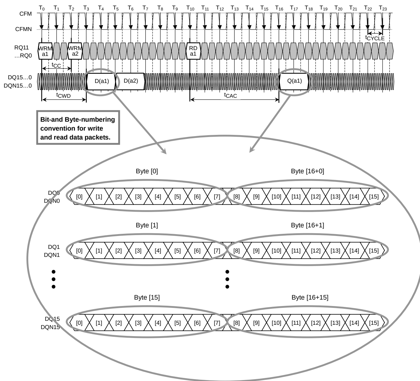
Figure 52. Write-Masked (WRM) Transaction Example
