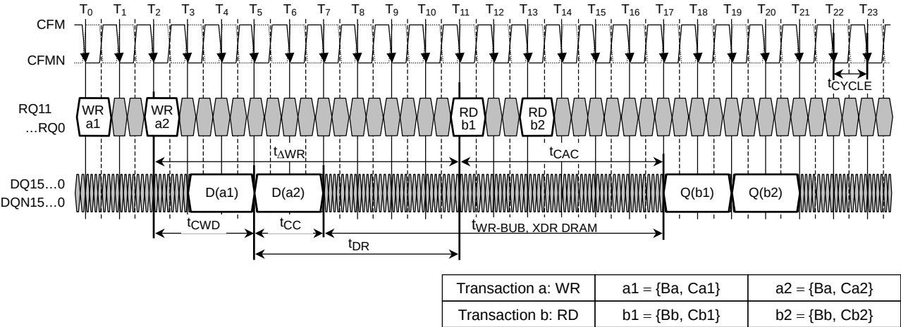
Write/Read Turnaround Example
