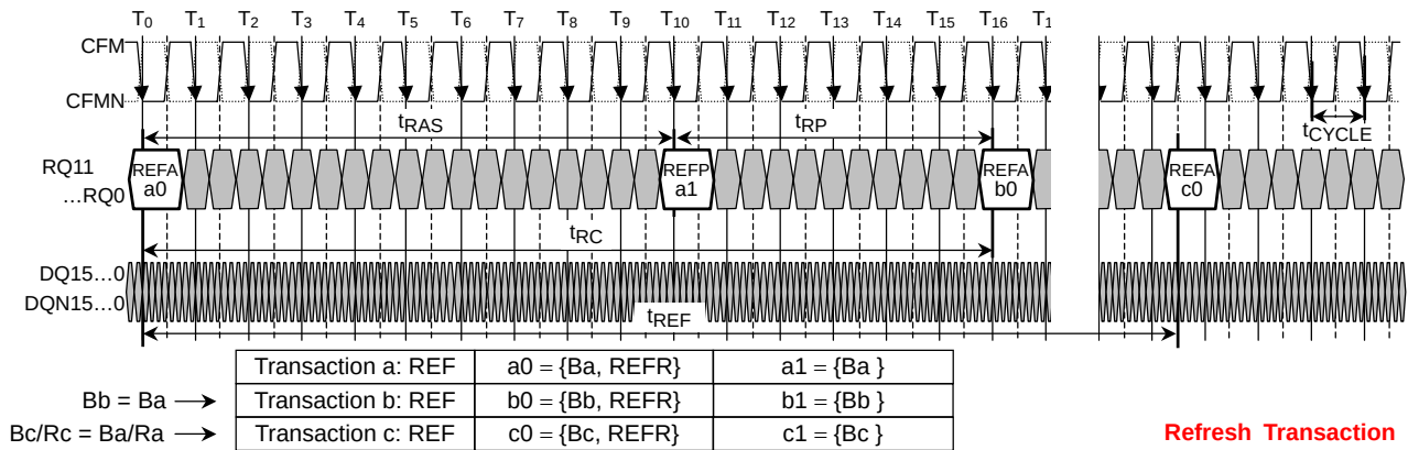
Figure 44. Refresh Transactions
