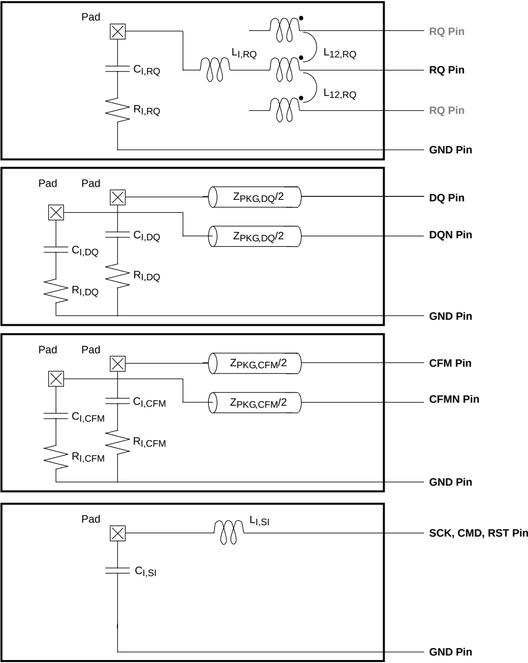
Figure 63. Equivalent Circuits for Package Parasitic
