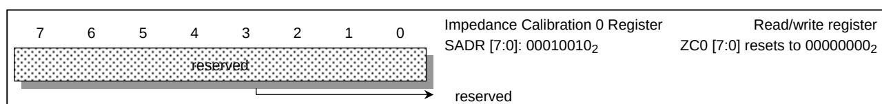
Figure 30. Impedance Calibration 0 (ZC0) Register
