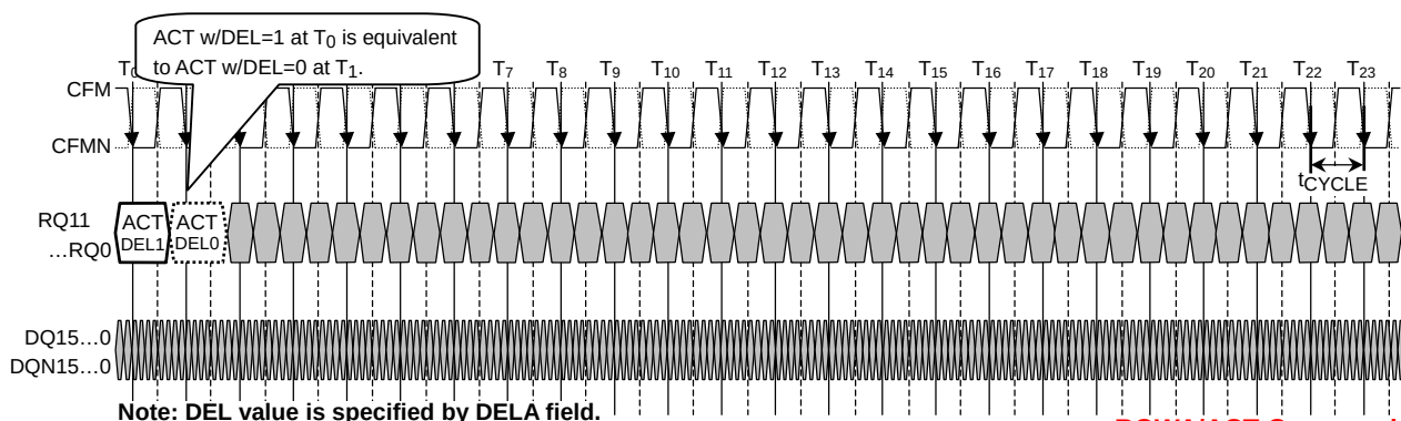
Figure 8. Request Scheduling Examples
