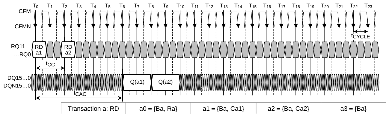
Figure 10. Read Transactions
