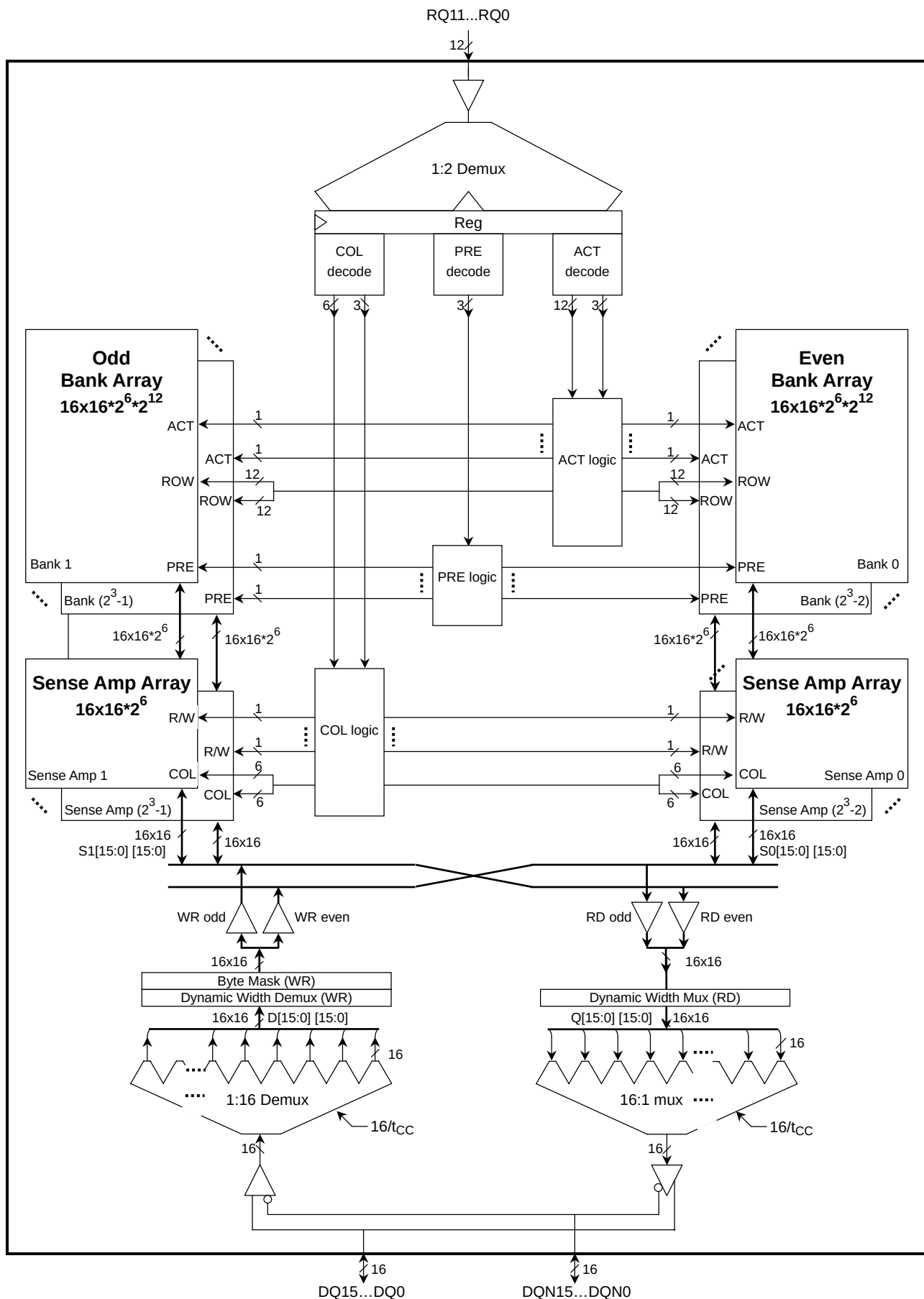
Figure 55. XDR DRAM Block Diagram with Bank Sets
