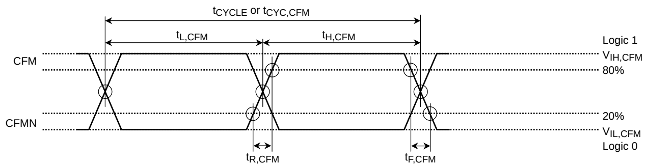
Figure 57. Clocking Waveforms
