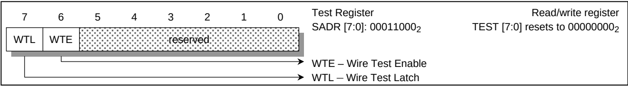
Figure 37. DLL Register
