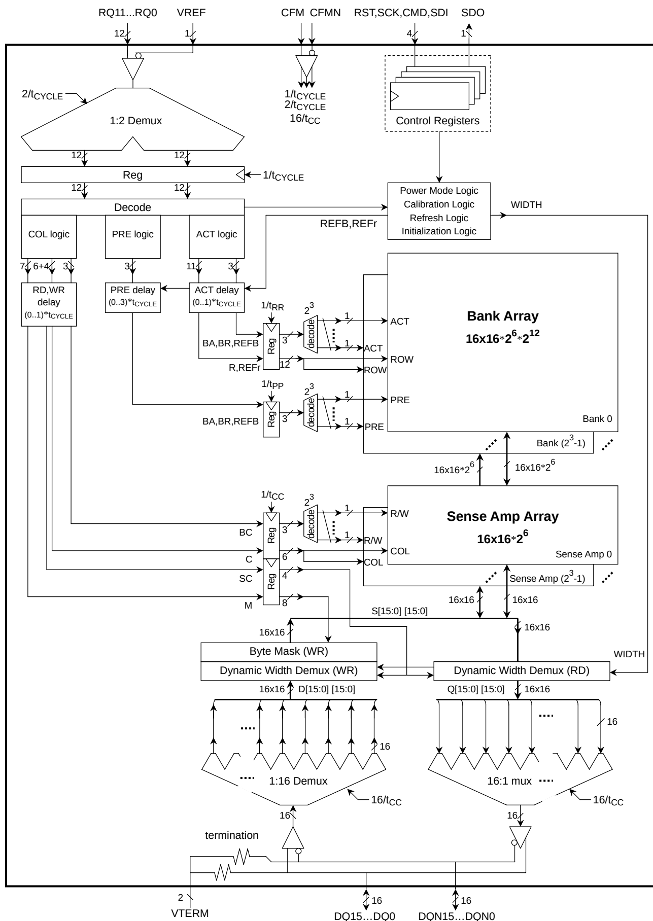
Figure 2. 256Mb (8x2Mx16) XDR DRAM Block Diagram
