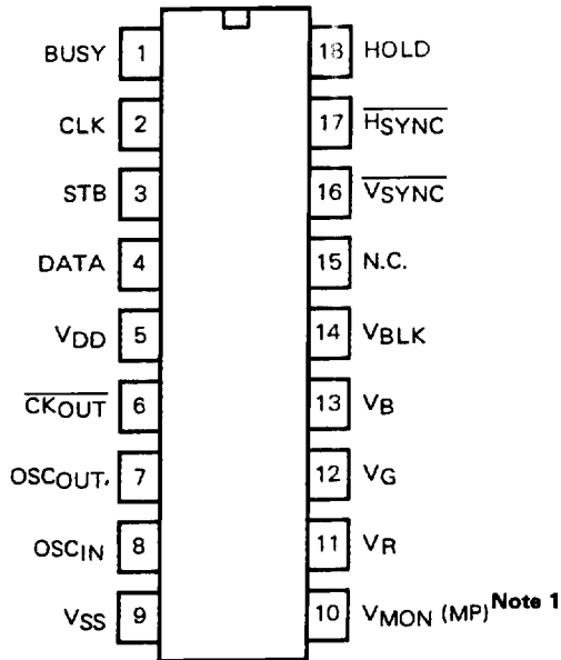
(1) \mu PD6451ACX-001
