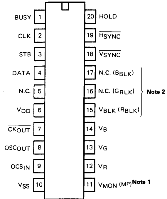
(2) \mu PD6451AGT-101
