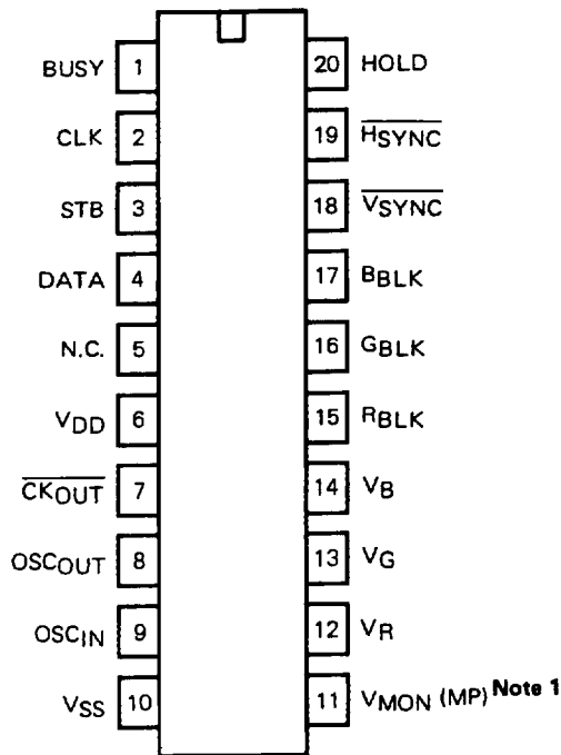
(3) \mu PD6451AGT-301
