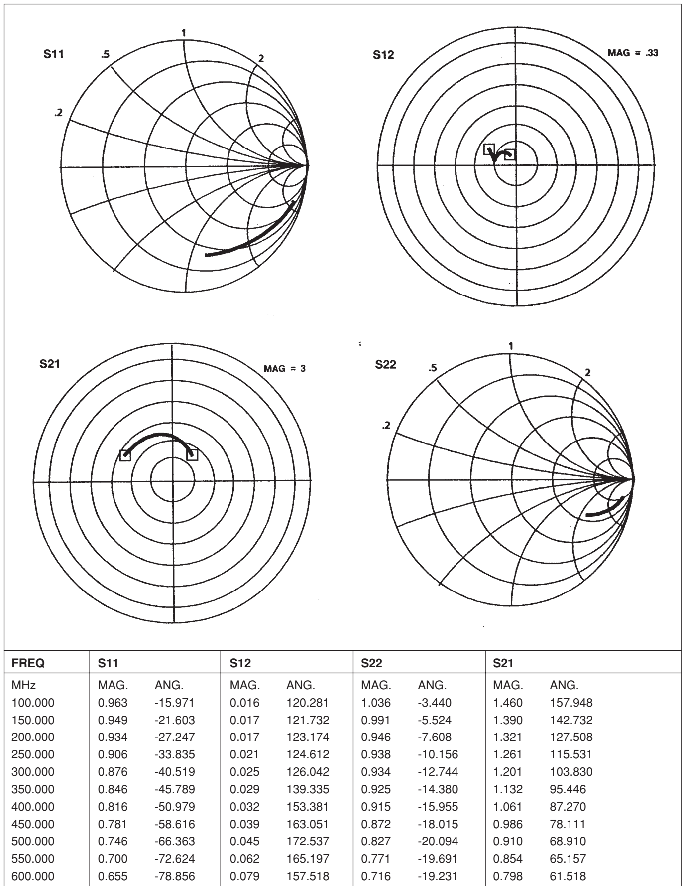
Figure 8: RF Amplifier
