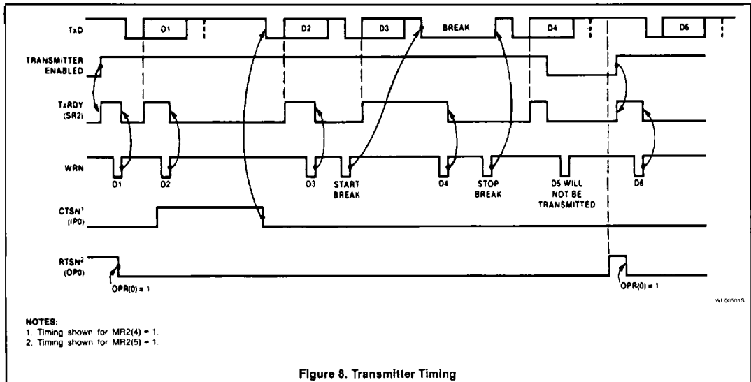
Figure 8. Transmitter Timing
