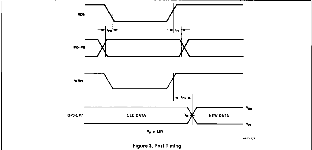
Figure 3. Port Timing
