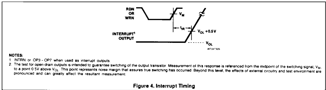
Figure 4. Interrupt Timing
