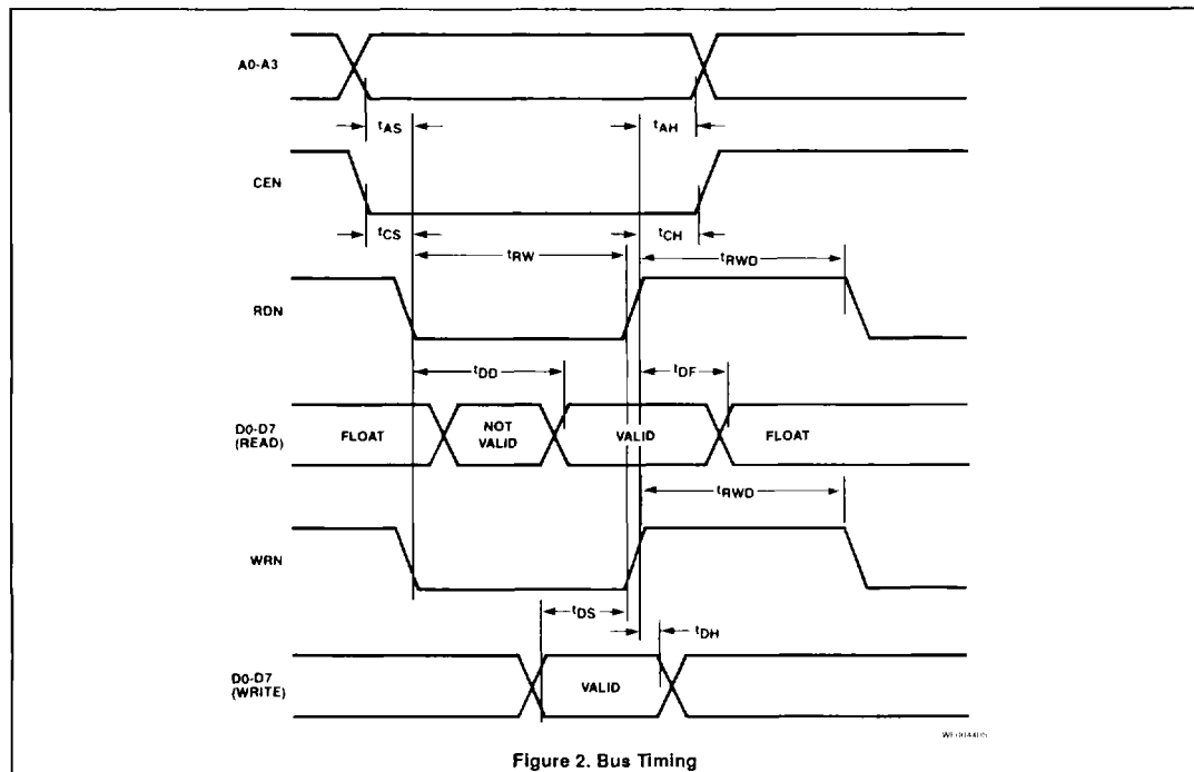
Figure 2. Bus Timing
