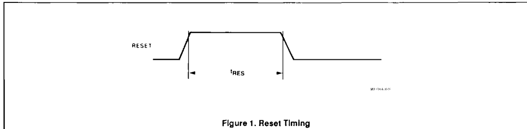
Figure 1. Reset Timing
