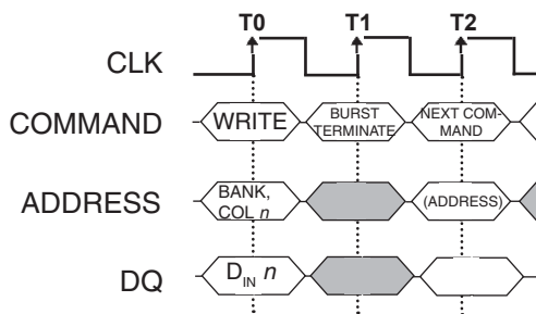
Figure 19 TERMINATING A WRITE BURST
