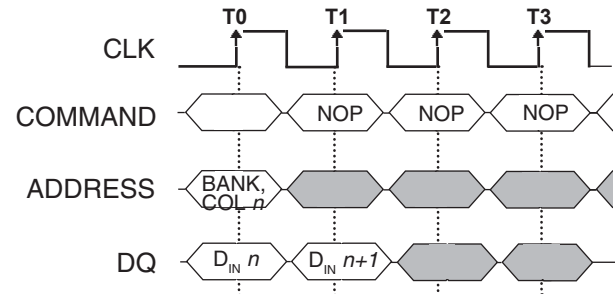
Figure 14 WRITE BURST
