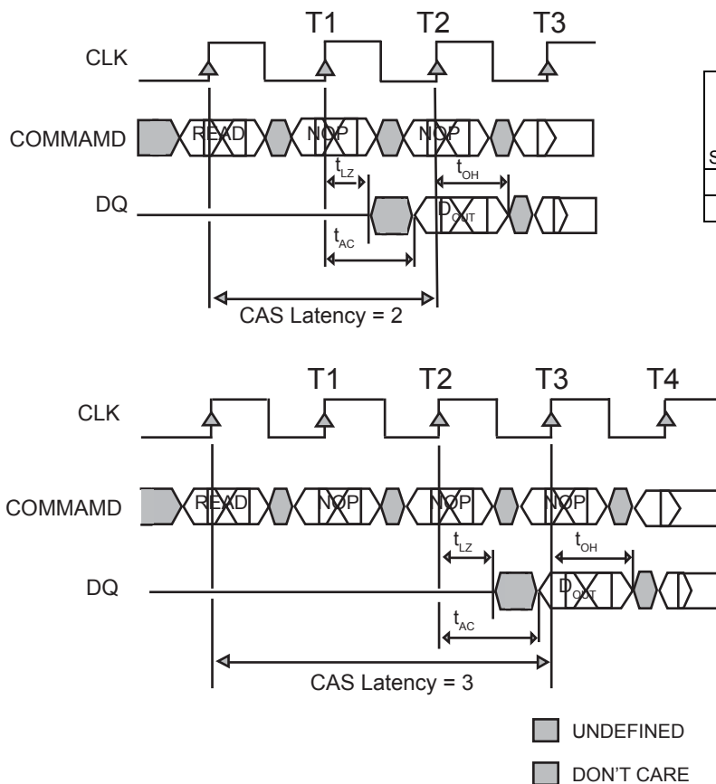
Figure 2 CAS LATENCY
