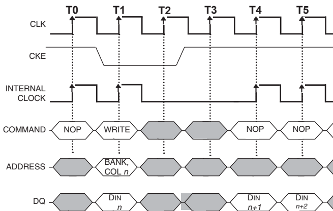
Figure 22 CLOCK SUSPEND DURING WRITE BURST
