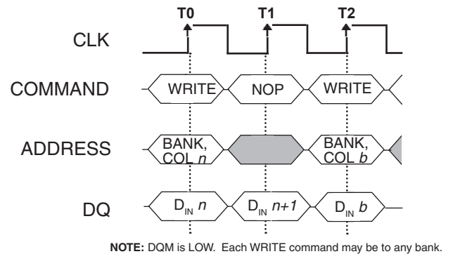
Figure 15 WRITE TO WRITE
