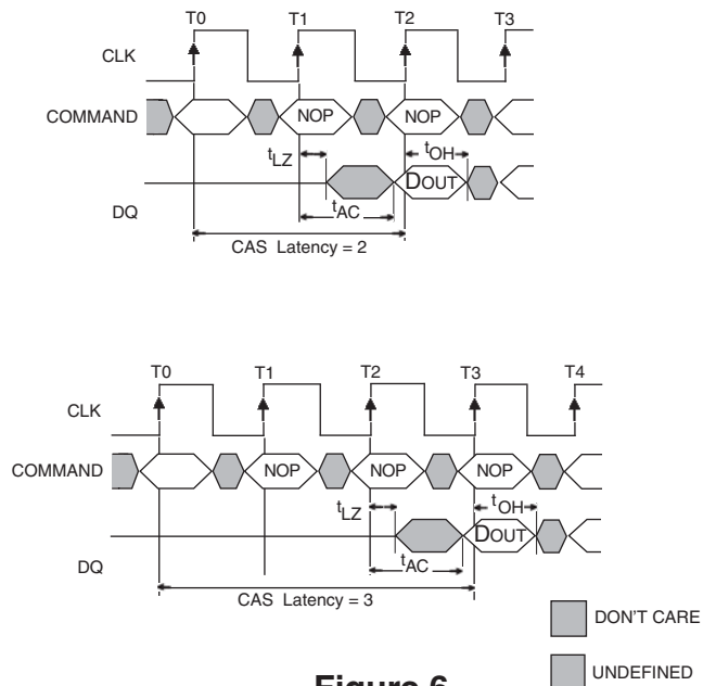
Figure 6 CAS LATENCY
