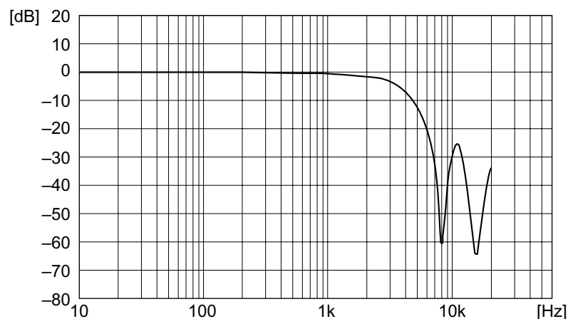
Figure 6 LPF Frequency Characteristics ( f_{SAM}=8 kHz)
