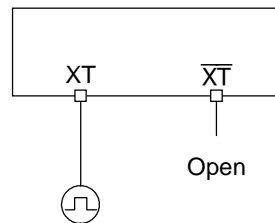
Figure 5 Oscillation Circuit using an external clock input
