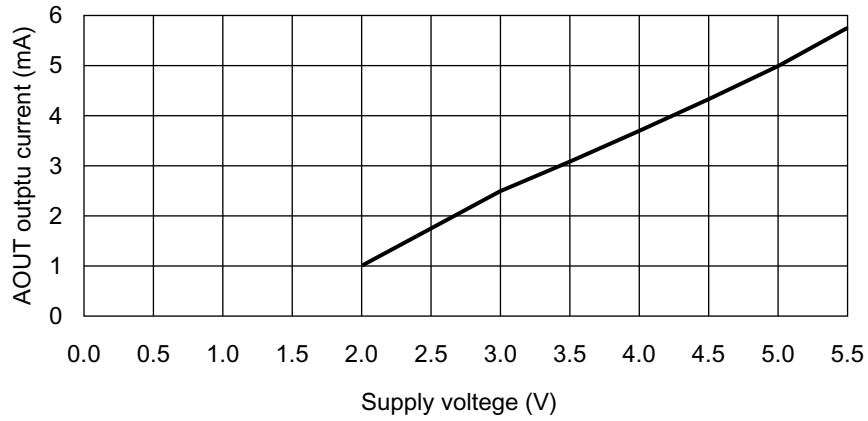
Relationship between supply voltage and AOUT output current ( T_a = 20^\circ\text{C} , V_{AOUT} = V_{DD} , PCM at maximum)
