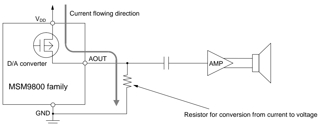
Circuit connection between the MSM9800 family product and amplifier IC
