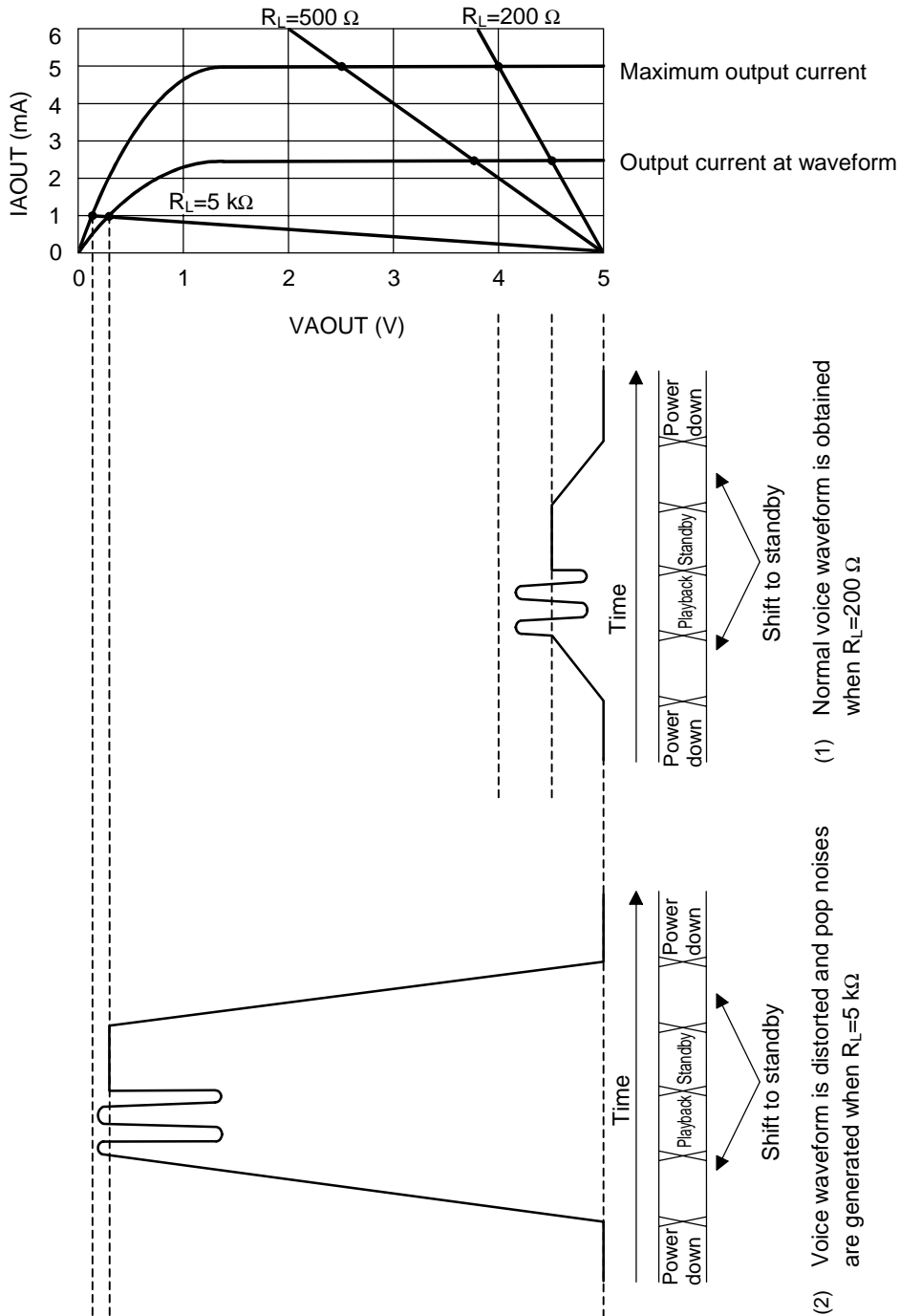
Relationship between AOUT pin voltage and AOUT output current at V_{DD} = 5 \text{ V}
