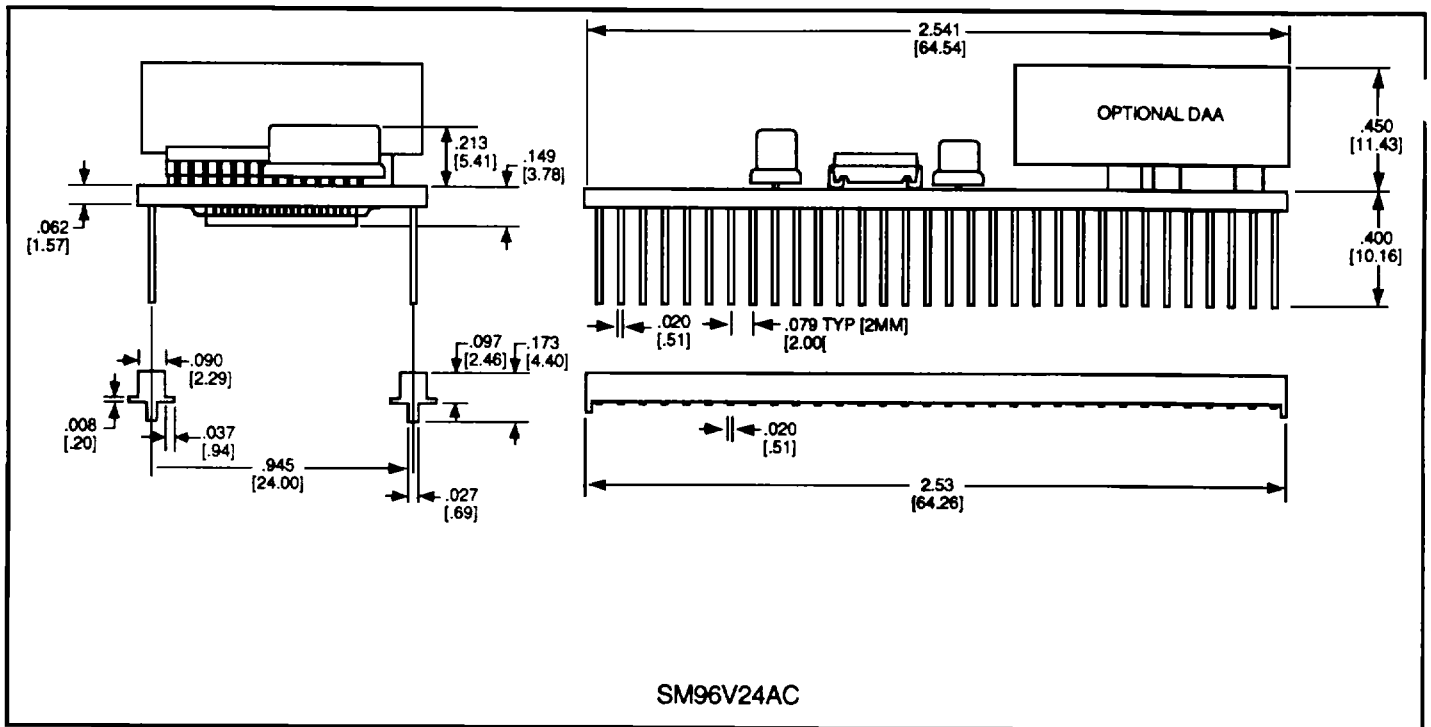
Figure 5. SM96V24AC Physical Dimensions
