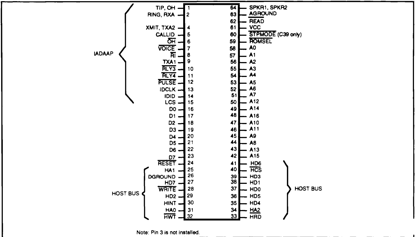
Figure 4. Parallel Pinout
