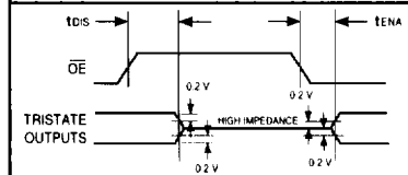
FIGURE 4. THRESHOLD LEVELS
