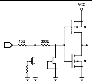
FIGURE 2. INPUT CIRCUIT
