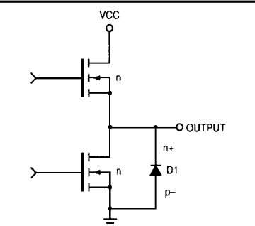
FIGURE 3. OUTPUT CIRCUIT
