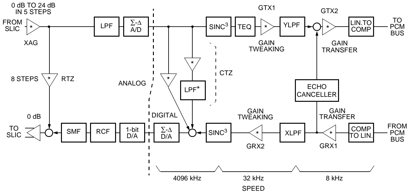
Figure 19. Internal Signal Processing
