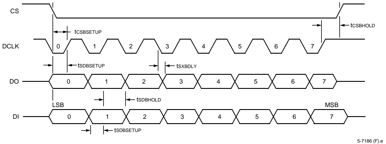
Figure 21. Serial Interface Timing, Byte-by-Byte Mode (One Byte Transfer and Gapped DCLK Shown)
