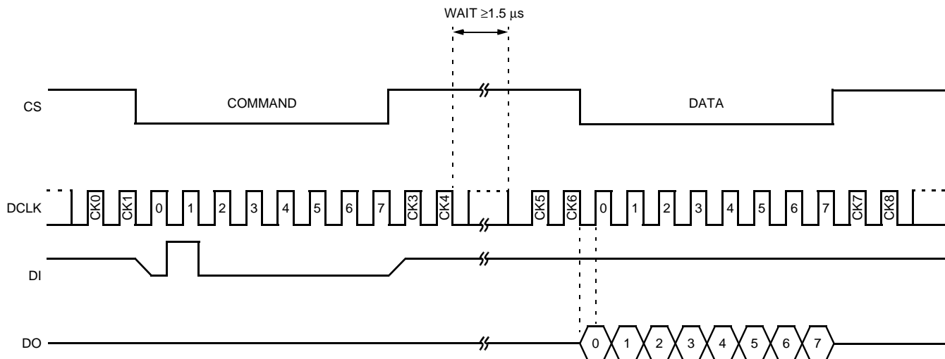
Figure 16. Fast Scan, Byte-by-Byte Mode (Continuous DCLK)
