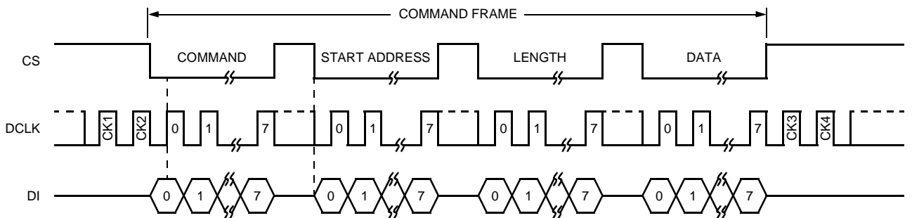
Figure 8. Write Operation, Byte-by-Byte Mode (Continuous DCLK)
