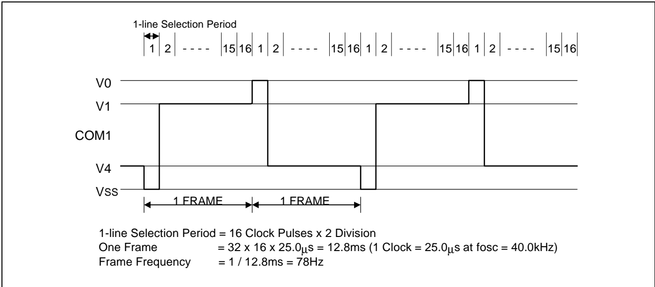
Figure 17. Frame Frequency
