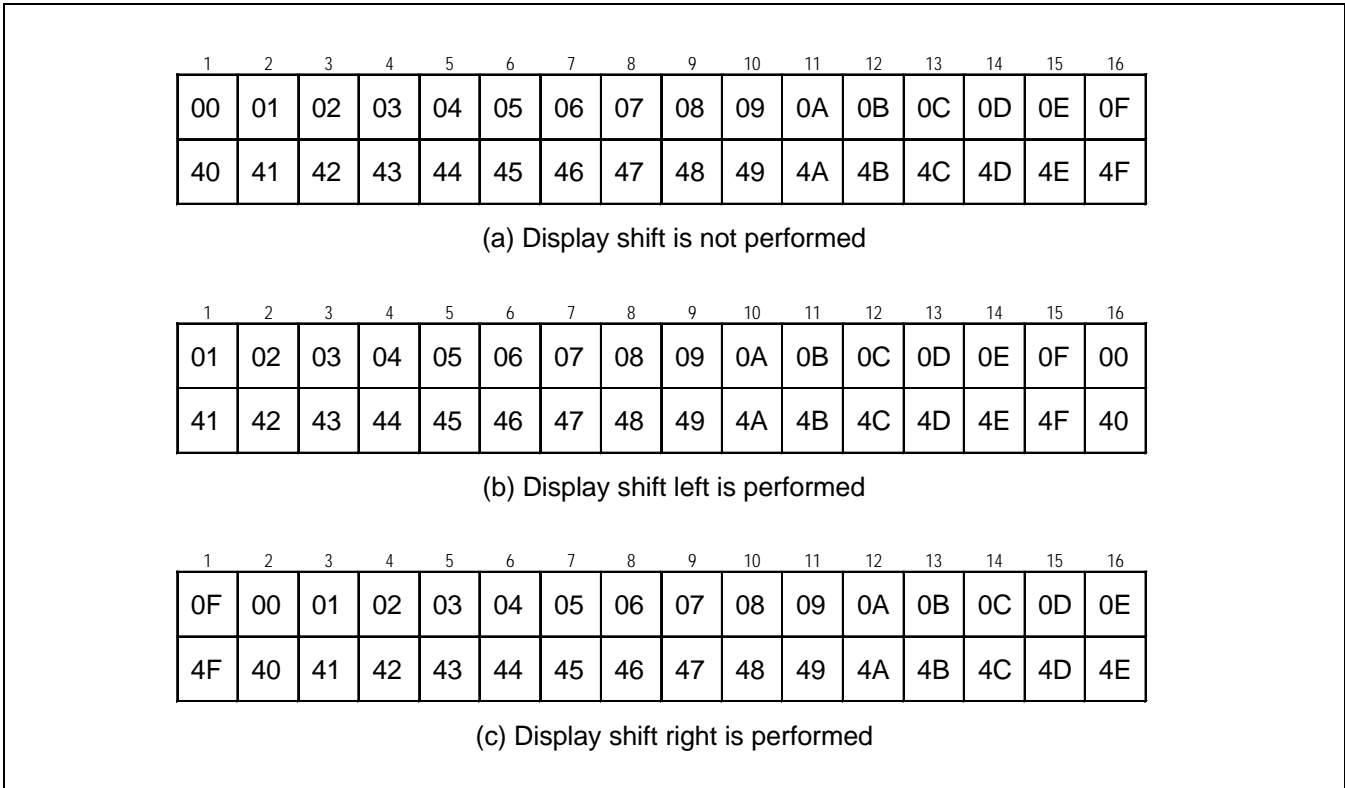
Figure 7. DDRAM Address
