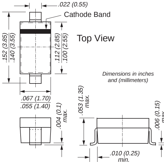
SOD-123
