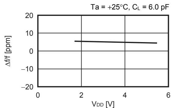
8. Crystal oscillator frequency deviation vs. Power supply voltage characteristics
