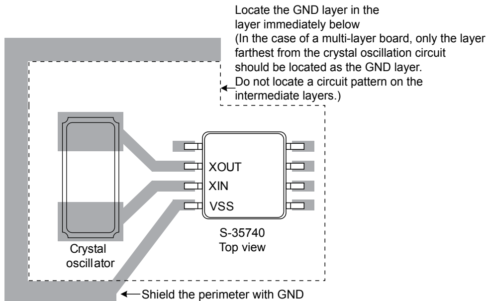
Figure 32 Example of Recommended Connection Pattern Diagram
