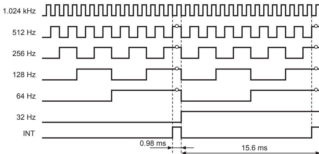
Figure 12 Example of Fixed-cycle Interrupt Signal Output (CMOS output)
