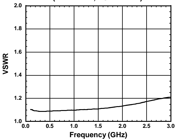
P1 VSWR vs. Frequency ( VDD=2.7V, VCTL=2.7V )
