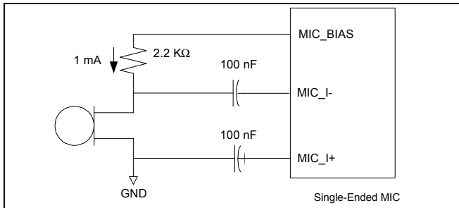
Figure 13. Single-Ended MIC
