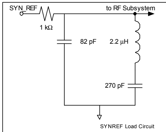
Figure 9. SYNREF Load Circuit
