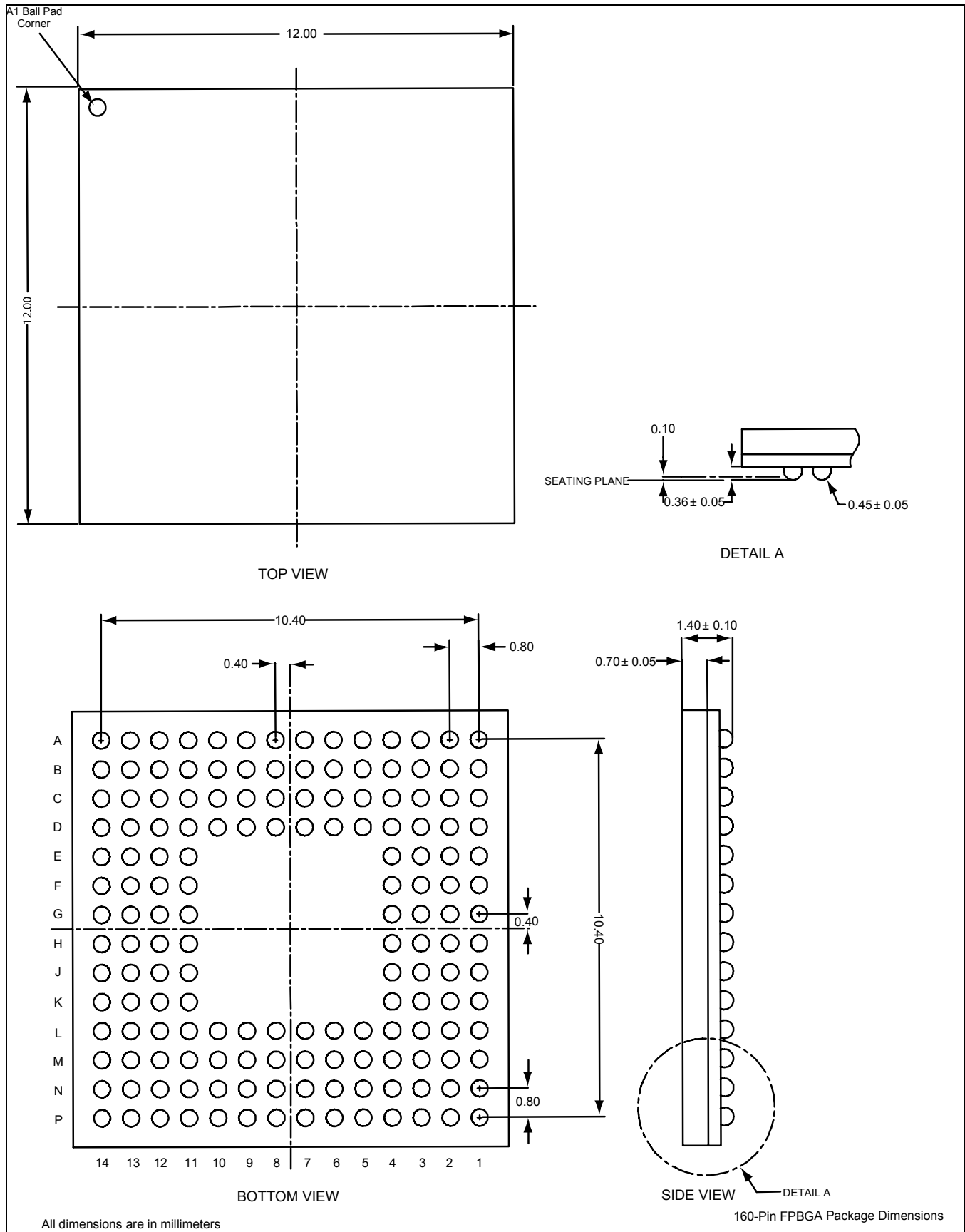
Figure 24. CX20524 160-Pin FPBGA Package Dimensions
