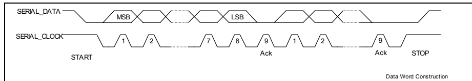
Figure 21. Data Word Construction
