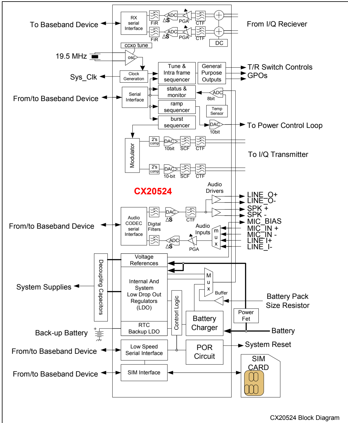
Figure 3. CX20524 Block Diagram
