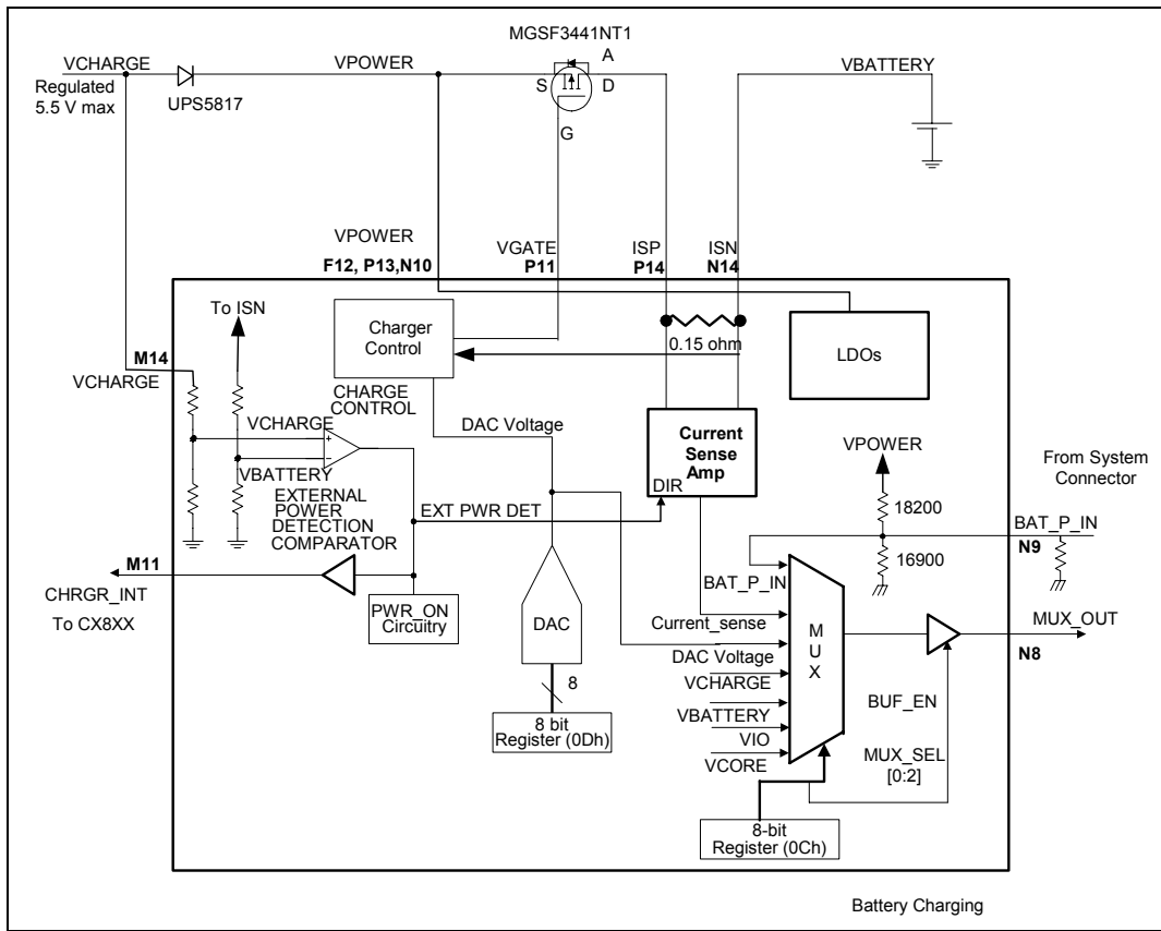
Figure 17. MSD Battery Charging
