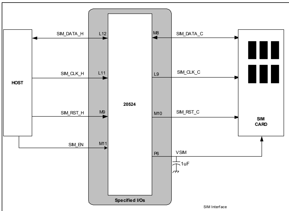
Figure 18. SIM Interface
