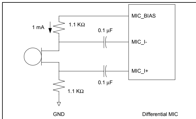
Figure 12. Differential MIC
