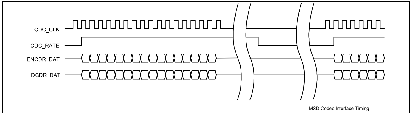
Figure 14. MSD Codec Interface Timing Diagram
