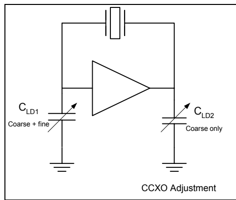
Figure 7. CCXO Adjustment
