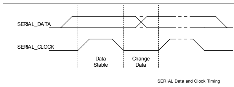
Figure 19. Serial Data and Clock Timing
