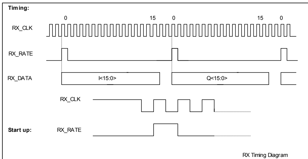
Figure 4. Receive Interface Timing Diagram
