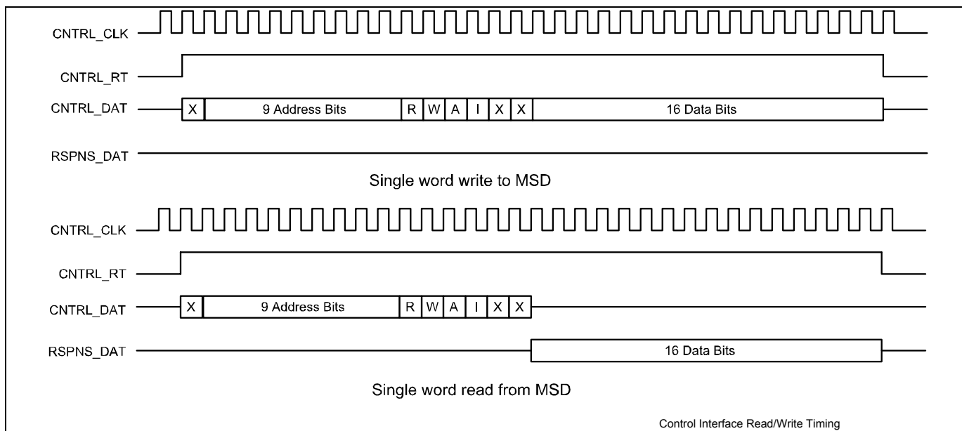
Figure 10. Control Interface Read/Write Timing Diagram
