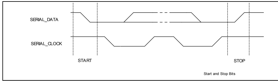
Figure 20. Start and Stop Bits
