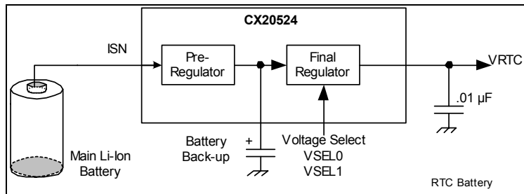
Figure 16. RTC Battery
