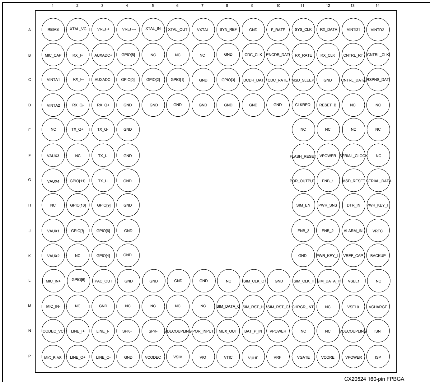
Figure 2. 160-Pin FPBGA Pinout – Top View
