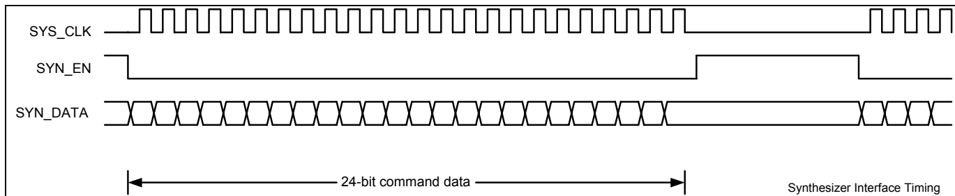
Figure 11. Synthesizer Interface Timing Diagram
