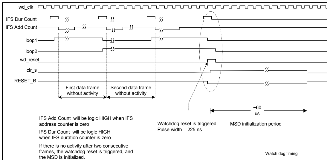
Figure 23. Watch Dog Timing
