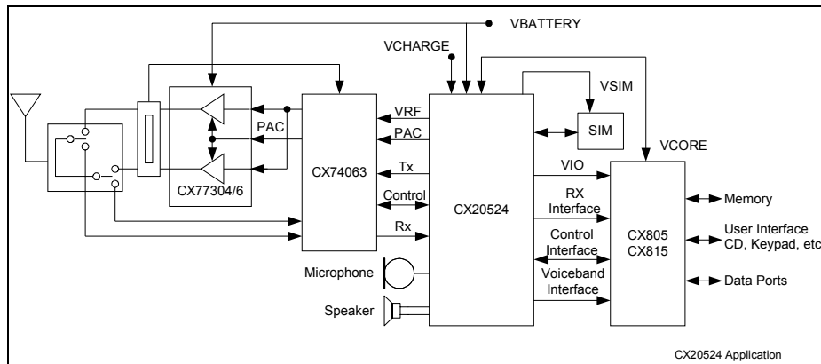
Figure 1. Typical CX20524 Application in a Handset Design
