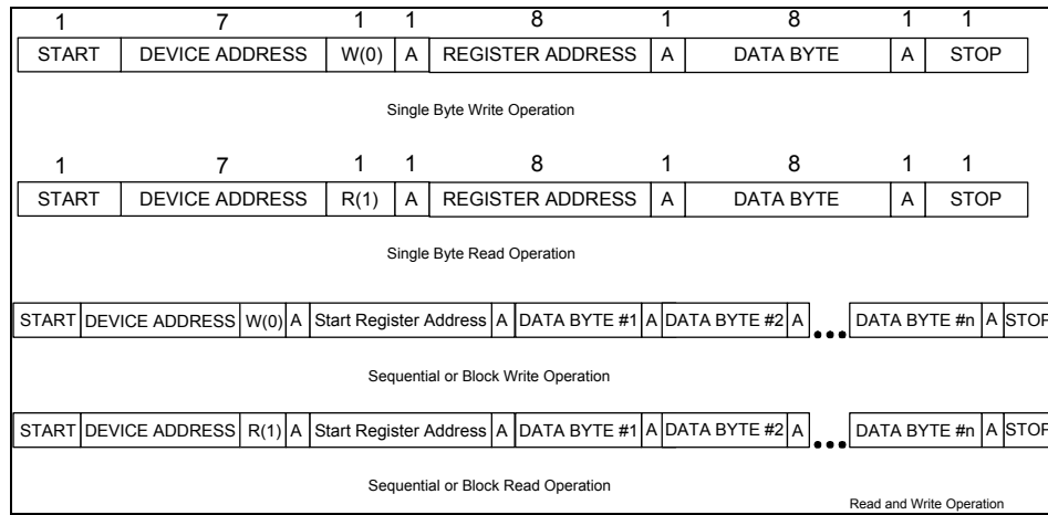
Figure 22. Sequential or Block Read/Write for Low Speed Asynchronous Serial Port
