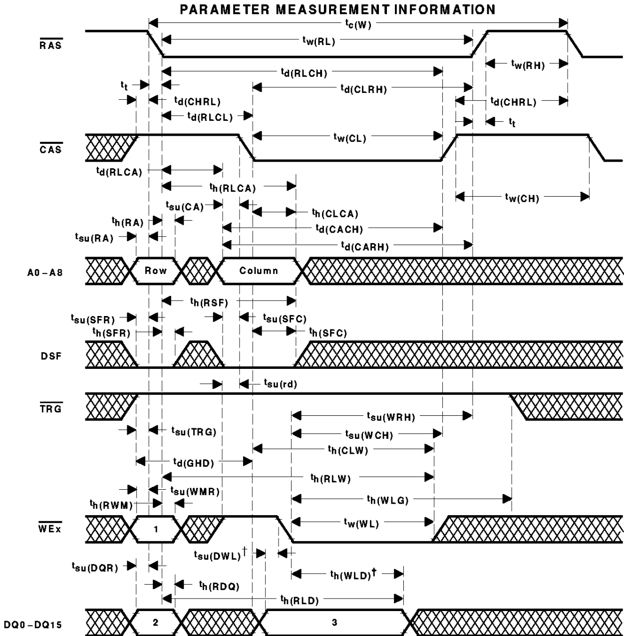
Figure 33. Late-Write-Cycle Timing (Output-Enable-Controlled Write)
