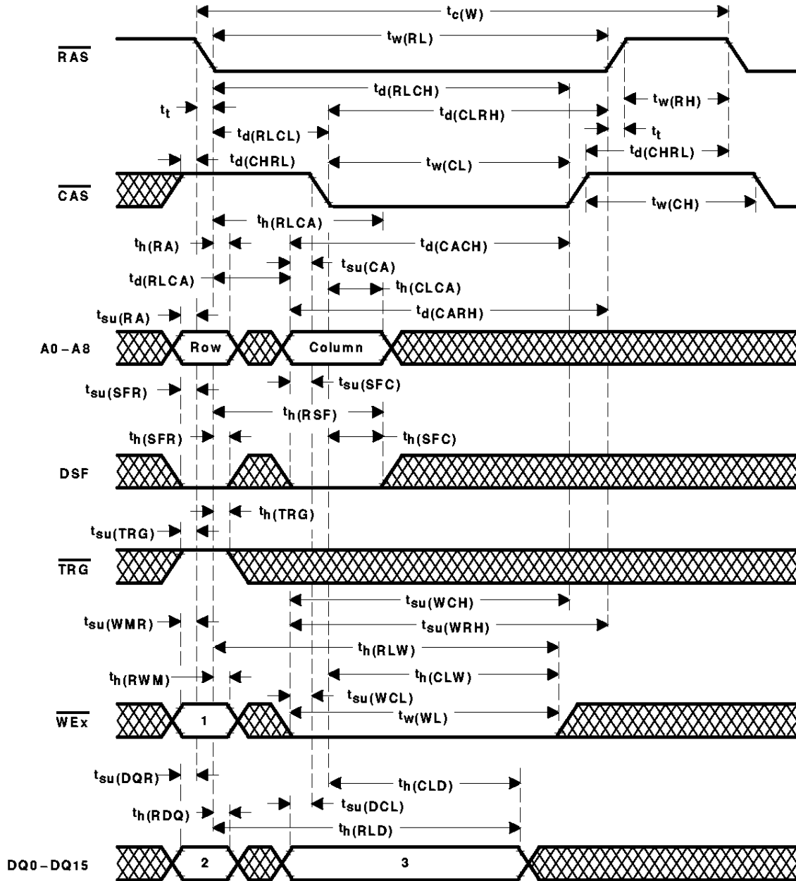
Figure 32. Early-Write-Cycle Timing
