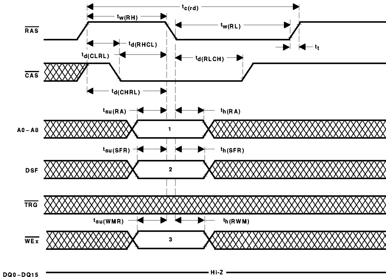
Figure 48. CBR-Refresh-Cycle Timing
