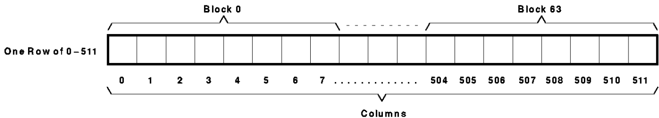
Figure 14. 8-Column-Block Column-Organization
