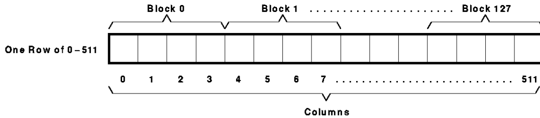
Figure 10. 4-Column-Block Column-Organization
