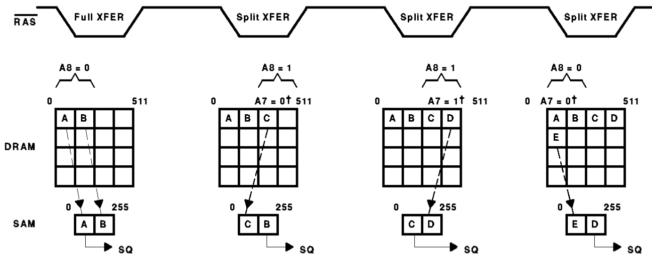
Figure 21. Example of a Split-Register-Transfer Read Operation
