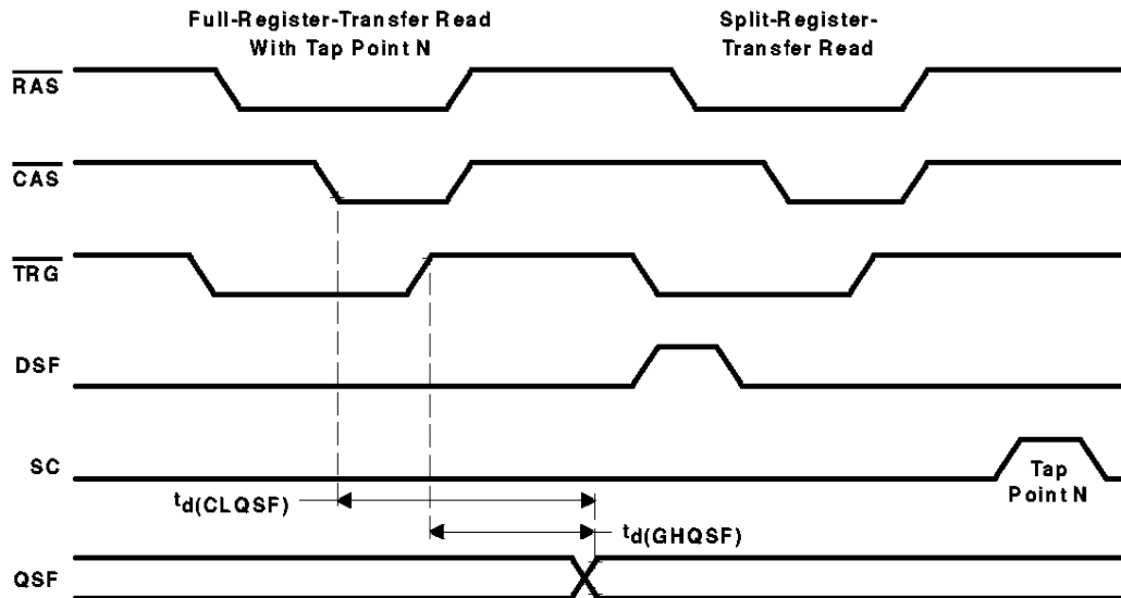
Figure 22. Example of a Split-Register-Transfer Read After a Full-Register-Transfer Read
