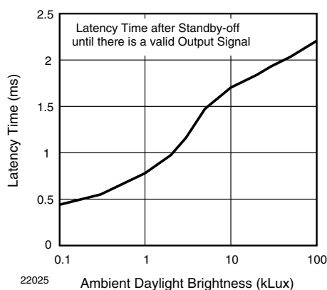
Fig. 19 - Delay Time after Standby-off until the TSOP75D25 is ready to receive Data
