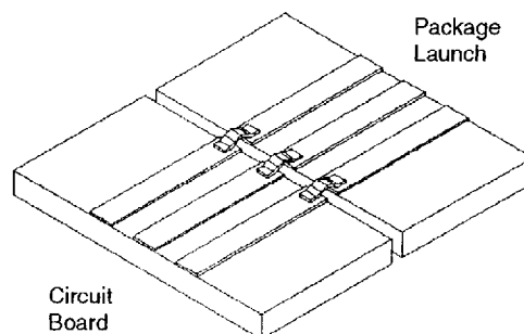
Figure 2. Microstrip Mount
