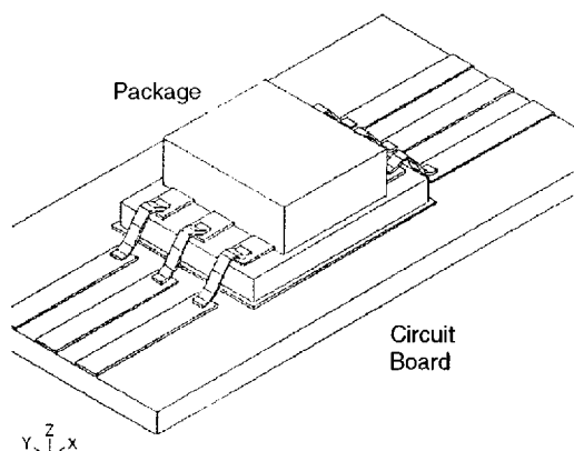
Figure 3. Surface Mount
