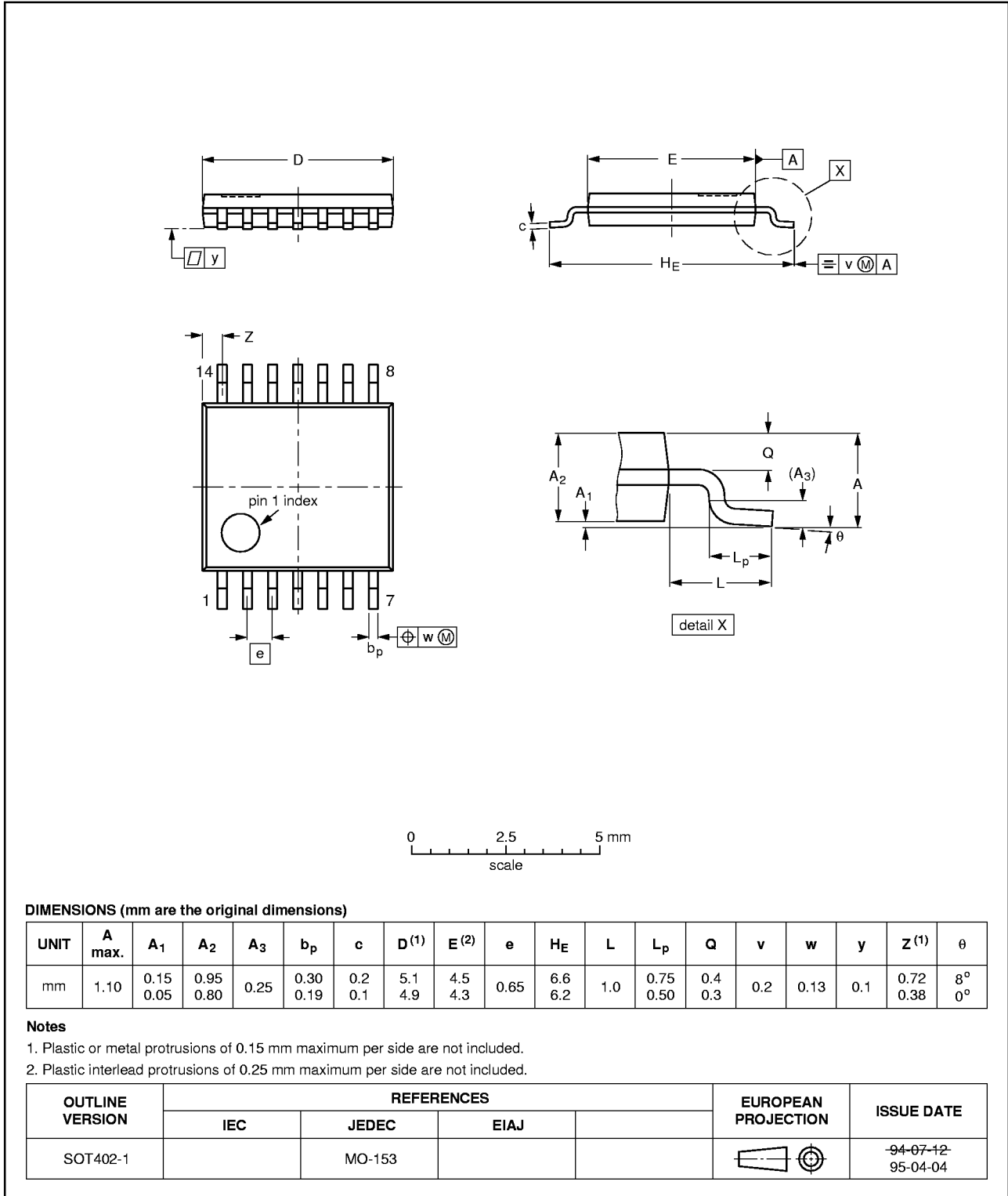
Fig 14. TSSOP14 package outline.
