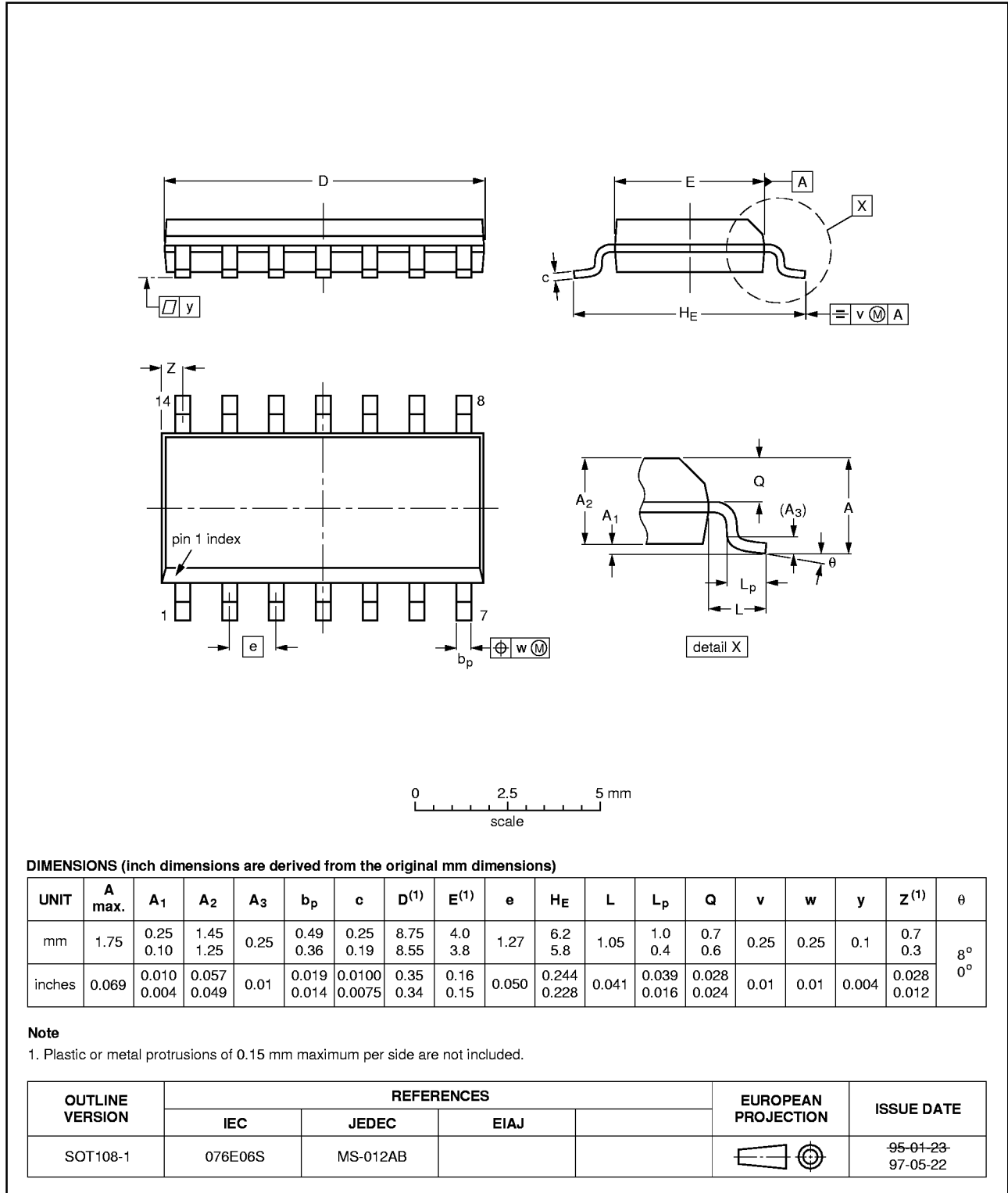
Fig 12. SO14 package outline.
