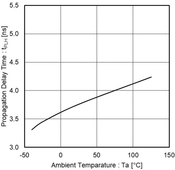
Figure 2. Propagation Delay Time: t PLH vs Ambient Temperature: Ta (V CC = 3.0 V)
