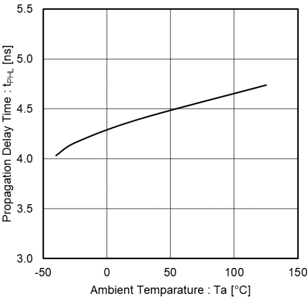
Figure 4. Propagation Delay Time: t PHL vs Ambient Temperature: Ta (V CC = 3.0 V)
